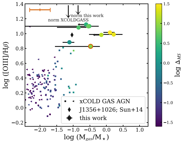
Figure 7. [O III] 5007 to H\beta emission-line ratio versus gas fraction ( M_{\text{gas}}/M_{\star} ) of our quasars (circles) and xCOLD GASS AGN (squares, with triangles for upper limits; from the catalogues provided with Saintonge et al. 2017). The errors on the [O III]/ H\beta ratios for our sample are smaller than the point size. A representative systematic error bar is shown in the top left-hand corner as in Fig. 6. J1010+0612 is highlighted with a red outline as per Fig. 5 and a black diamond marks the value for J1356+1026 using L'_{\text{CO}}(1-0) from Sun et al. (2014) instead of the limit from this work. Data points are colour-coded by their distance to the Sargent et al. (2014) main sequence ( \Delta_{\text{MS}} ). The two arrows show the average gas fraction from the Tacconi et al. (2018) sample matched in stellar mass and redshift to each population, to demonstrate that the observed trend is not dominated by differences in these parameters between the two samples. Sources with high [O III]/ H\beta ratios tend to have high gas fractions and have sSFRs above the main sequence.
