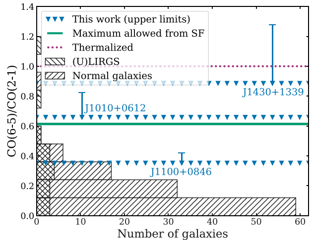
Figure 8. Upper limits of L'_{\text{CO}}(6-5)/L'_{\text{CO}}(2-1) ratios, for the three sources with these observations, represented as lines of blue triangles. Corresponding error bars represent the maximum values given the uncertainty on the measured CO(2–1) flux. The green line marks a maximum ratio achievable from star formation alone assuming a maximum SFR surface density of 1000 M_{\odot} \text{ yr}^{-1} \text{ kpc}^{-2} following Narayanan & Krumholz (2014). The dotted magenta line marks where the molecular gas becomes thermalized. The histograms show the distribution of L'_{\text{CO}}(6-5)/\text{CO}(2-1) ratios for literature galaxy samples from Papadopoulos et al. (2012) ([U]LIRGs only) and Kamenetzky et al. (2016). For at least two of our sources (J1010+0612 and J1100+0846), we do not have any evidence for highly excited CO SLEDs (see Section 5.2).
