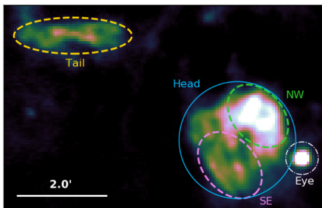
Figure 7. Tornado head and tail region at 70\ \mu\text{m} . The shapes indicate regions from which we detect FIR emission and within which we compare the flux ratios in Figs. 9 and 10. These are the Tornado head (blue circle), north-western head (green dashed ellipse), south eastern head (pink dashed ellipse), Tornado tail (gold dashed ellipse), and the Tornado eye (white dash-dotted circle).
