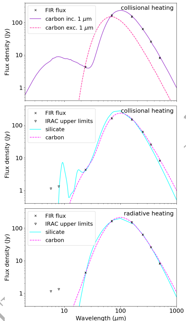
Figure 8. Best-fit dust SEDs for the Tornado head assuming that dust is collisionally heated by hot gas in the top two panels, and radiatively heated in the bottom panel. We use DINAMO ( Priestley et al. 2019 ) to fit to the flux within the head aperture in Fig. 7, assuming the gas properties estimated by ( Sawada et al. 2011 ). Although we can fit the SED well to the measured FIR fluxes with a collisional heating model and carbon grains, this requires a highly unusual grain size distribution. It is more likely that the majority of the dust within the Tornado head is radiatively heated, with a small proportion of collisionally heated dust.
