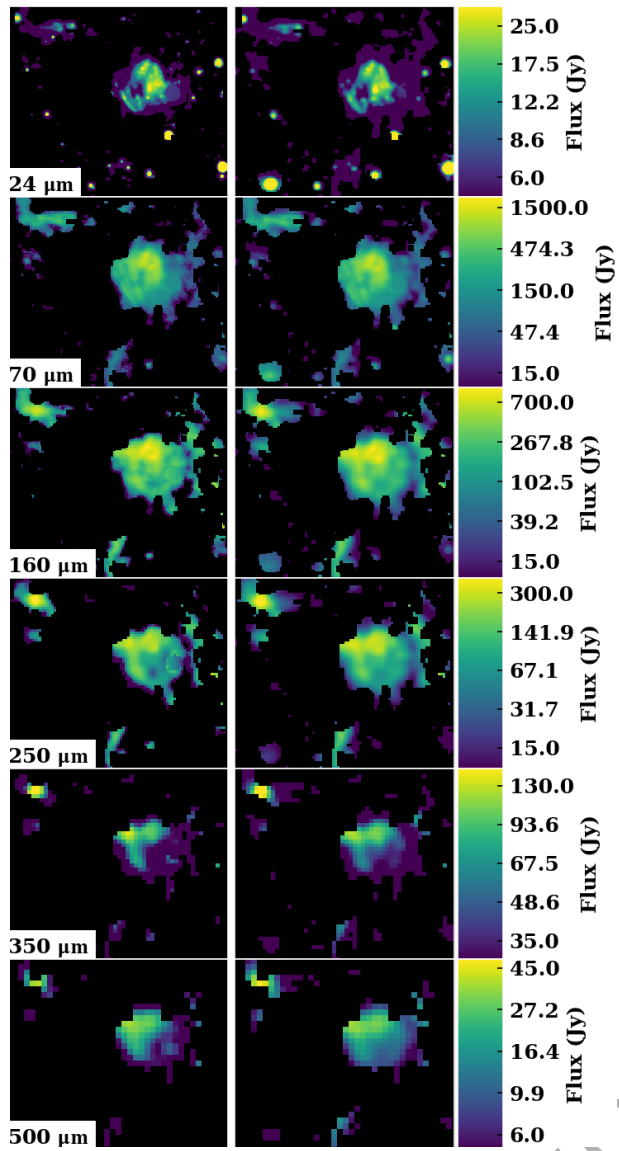
Figure A1. A grid comparing the original Spitzer and Herschel observations of the Tornado ( left ) with the synthetic observations ( right ) created by taking the results from PPMAP and post-processing them.
