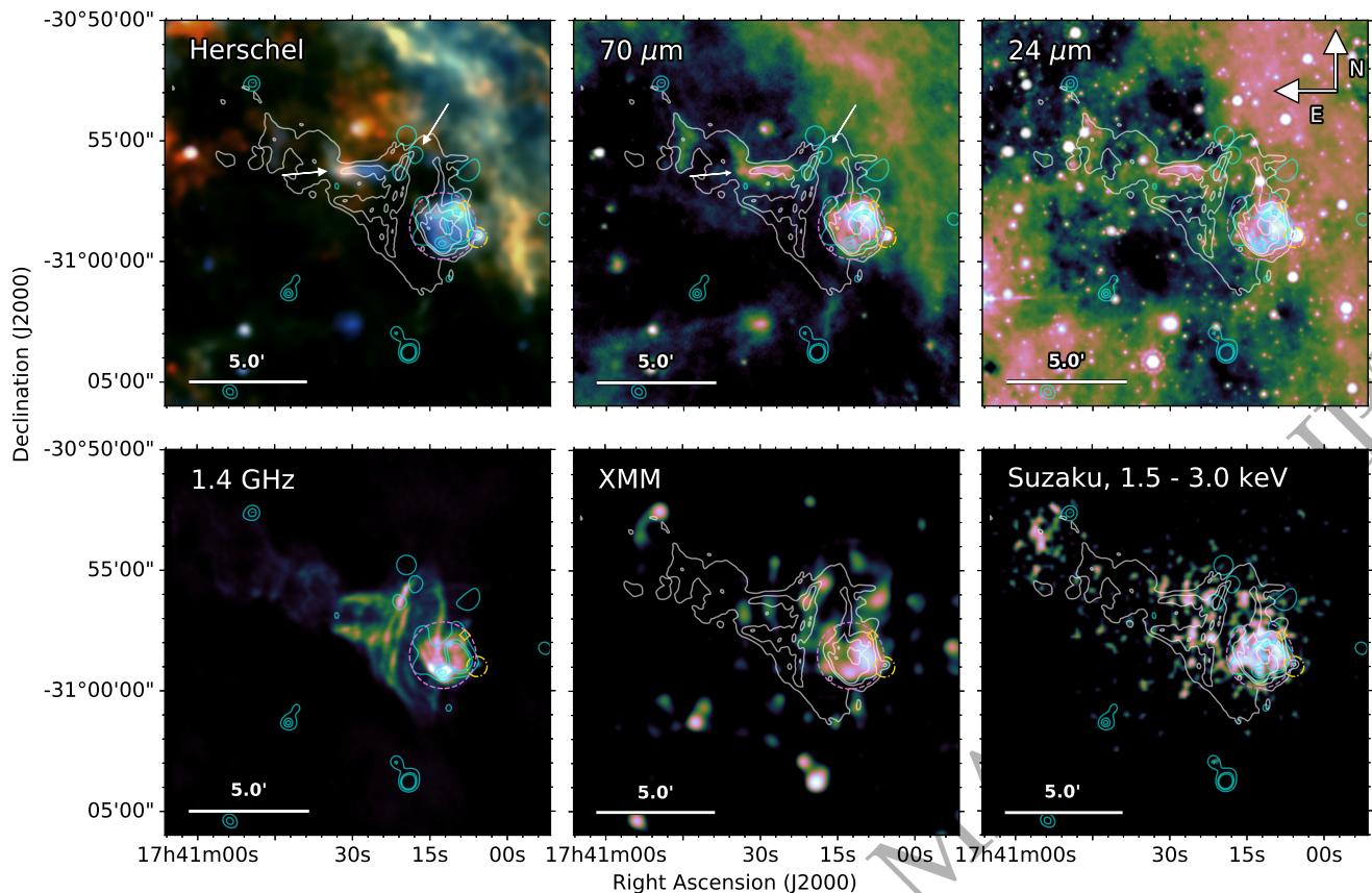
Figure 2. G357.7–0.1, The Tornado at FIR, radio, and X-ray - top left: Herschel three colour image made by combining the 70 (blue), 160 (green) and 250 \mu\text{m} (red) images, top middle: Herschel 70 \mu\text{m} image, top right: Spitzer MIPS 24 \mu\text{m} image, bottom left: 1.4 GHz VLA image, bottom middle: XMM-Newton X-ray image smoothed to 0.5'' pixels (kindly provided by B. Gaensler et al. private communication), and bottom right: Suzaku 1.5–3.0 keV X-ray smoothed continuum image. The white contours show the radio emission (1.4 GHz VLA) and the cyan contours show X-ray emission ( XMM-Newton ). We detect dust emission across all Herschel wavebands from the ‘head’ of the Tornado, within the pink circle. We also detect FIR emission from the ‘tail’ of the Tornado, and from a fainter filament extending around the head, as indicated by the arrows. The gold diamond indicates the location of an OH (1720 MHz) maser. (For the single wavelength panels we use the CUBEHELIX colour scheme, Green (2011).)
