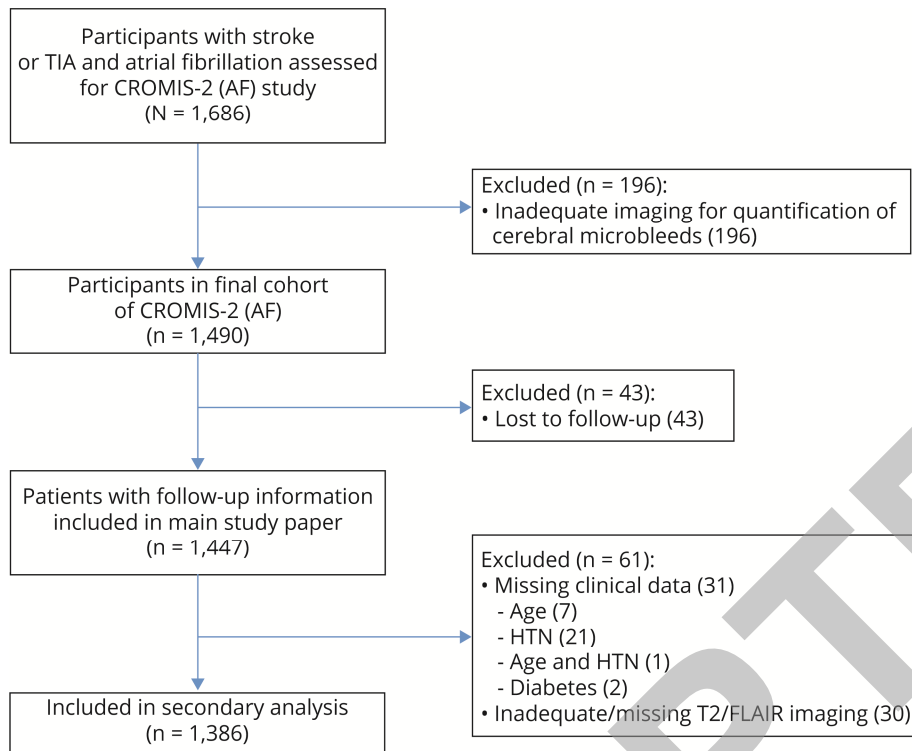
Figure 1: Study flowchart
