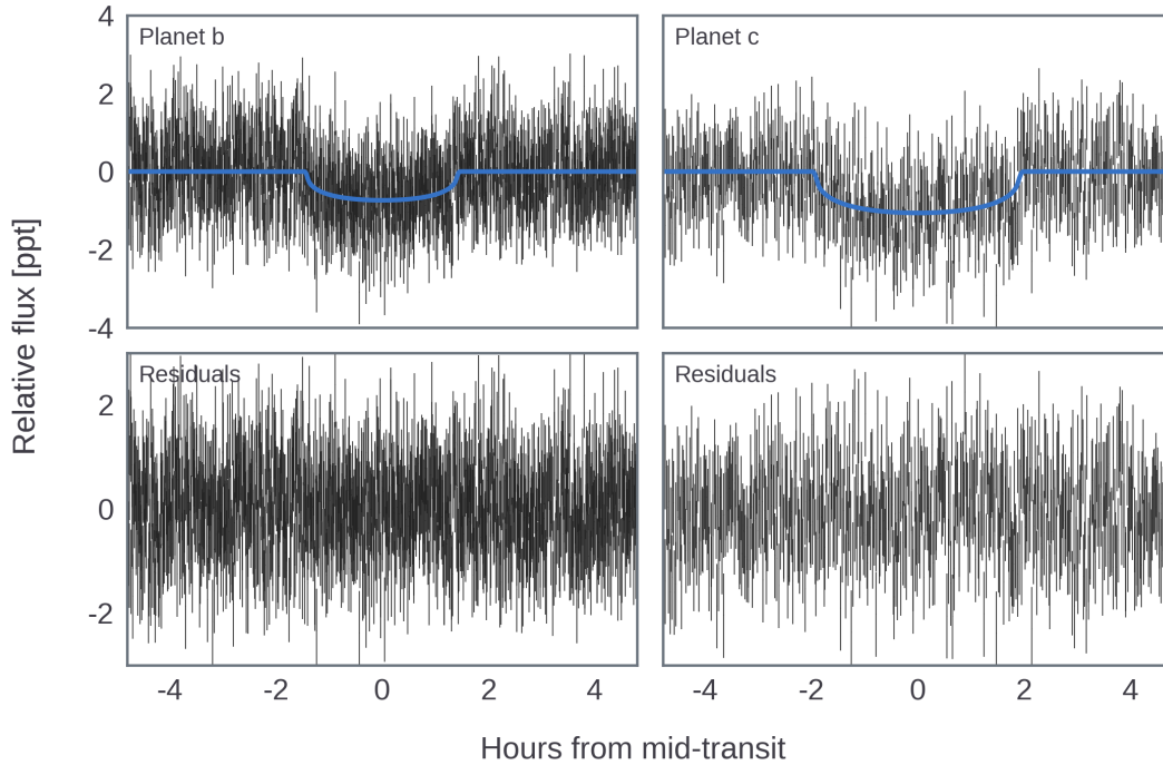
Figure 3. Flattened TESS photometry (black) folded on the best-fitting orbital periods of the two transiting planets, with transit models overlotted in blue (Sect. 5).
