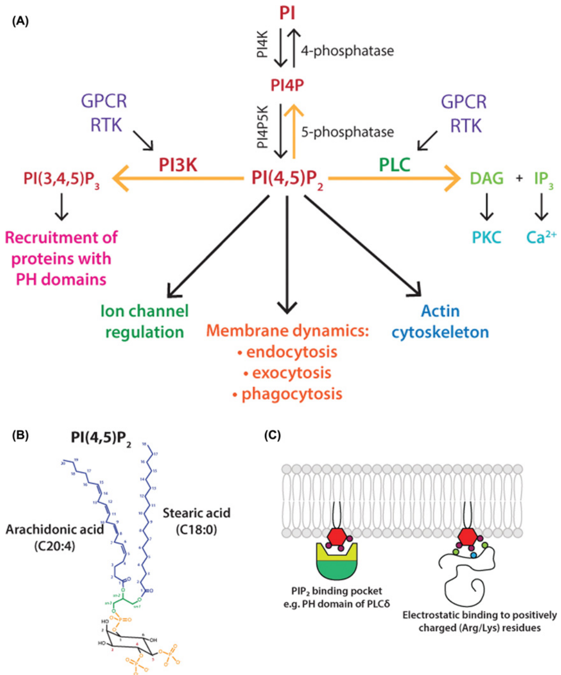
Figure 1. Phosphatidylinositol(4,5)bisphosphate (PI(4,5)P 2 )
