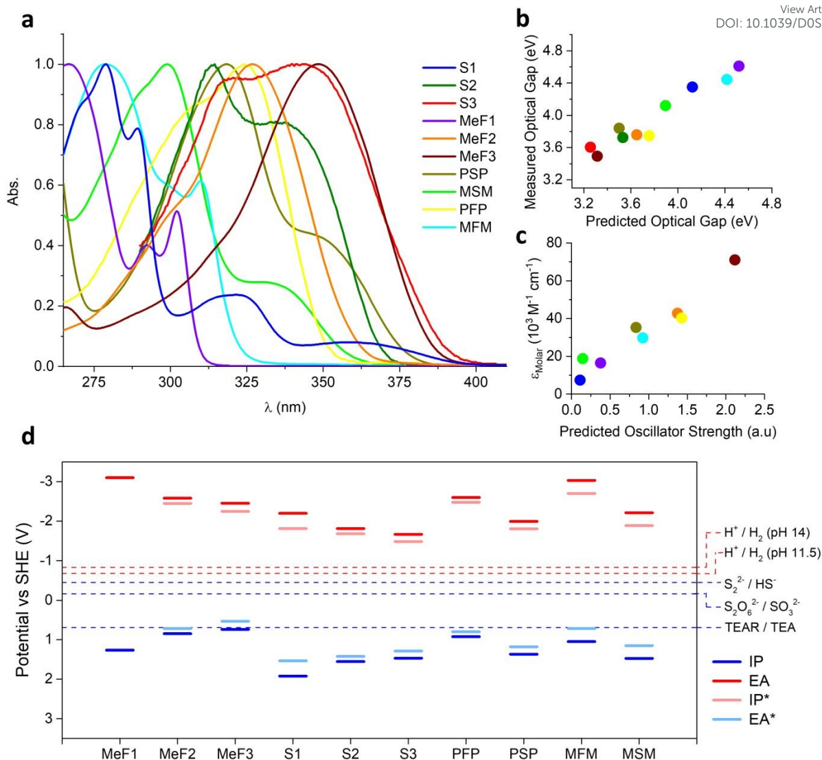
Figure 3. a) UV-Vis absorption spectra of the oligomers in chloroform; b) Plot of the TD-DFT predicted optical gap versus the value obtained from absorption maxima in chloroform solution; c) Plot of the oscillator strength predicted by TD-DFT versus the measured molar extinction coefficient ( \epsilon_{\text{Molar}} ) in chloroform solution; d) Potentials of the free charge carriers (IP,EA) and excitons (IP*,EA*) in the studied oligomers predicted by DFT and relevant solution reactions (at pH 11.5 for the case of using triethylamine as hole scavenger and pH 14.0 in the case of \text{SO}_3^{2-} and \text{HS}^- ). Potential of the 2-hole oxidation of triethylamine to diethylamine and acetaldehyde not shown as it lies in a similar place as the proton reduction potential for pH 11.5.
