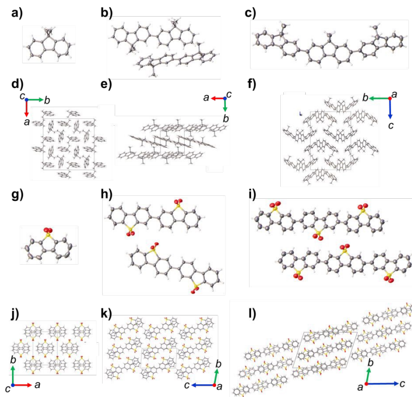
Figure 2. Displacement ellipsoid plots from the single crystal structures of; a) MeF1, b) MeF2, c) MeF3, g) S1, h) S2, i) S3; ellipsoids displayed at 50% probability level. Crystal packing in the single crystal structures of; d) MeF1, e) MeF2, f) MeF3, j) S1, k) S2, l) S3. Grey = carbon, white = hydrogen, yellow = sulfur; red = oxygen.
