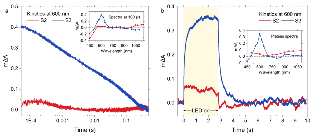
Figure 5. Optical signals from photogenerated charges under transient or quasi-continuous illumination, probed at 600 nm for suspensions of S2 and S3 in TEA/MeOH/water. (a) Transient absorption decay kinetics following laser excitation (pulse duration 4-7 ns), and (b) photoinduced absorption kinetics showing charge accumulation during illumination with a 2.7 s LED pulse and charge decay once the LED is turned off. The insets show the corresponding spectra, probed (a) at 100 \mu s under transient conditions and (b) at the plateau under quasi-continuous illumination. Excitation conditions: 355 nm, 0.40 \text{mJ cm}^{-2} for laser; 365 nm, 5.5 \text{mW cm}^{-2} for LED.
