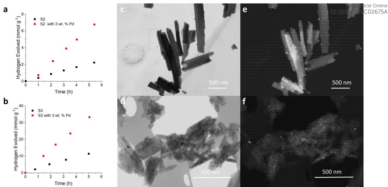
Figure 4. Hydrogen evolution of (a) S2 (5 mg) and (b) S3 (5 mg) in TEA/MeOH/water (1:1:1, 5 mL) with and without the addition of 3 wt. % Pd by photodeposition of [\text{Pd}(\text{NH}_4)_2\text{Cl}_4] , irradiated with a 300 W Xe light source fitted with a \lambda > 295 nm filter. STEM images of S2 with 3 wt. % Pd in (c) bright field mode and (e) high angle dark field mode and S3 with 3 wt. % Pd in (d) bright field mode and (f) high angle dark field mode.
