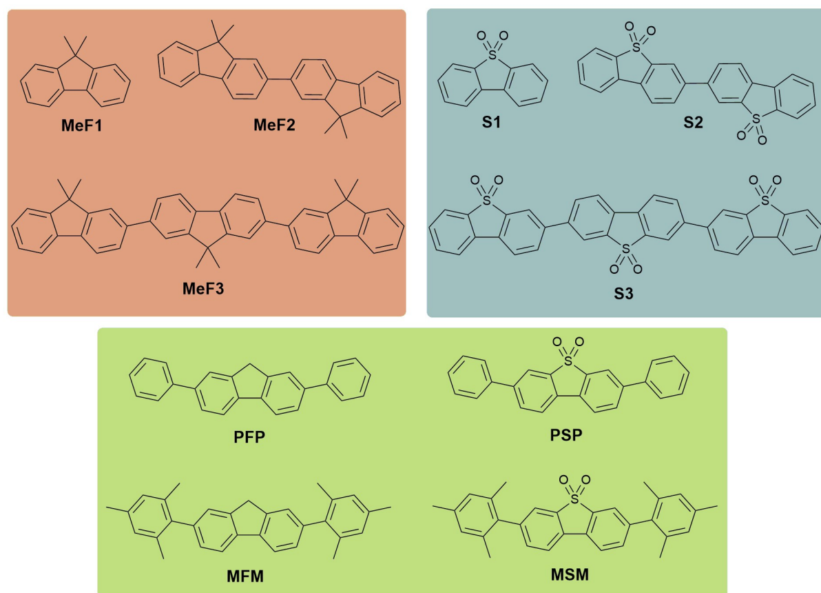
Figure 1. Structures of the oligomer photocatalysts in this study.
