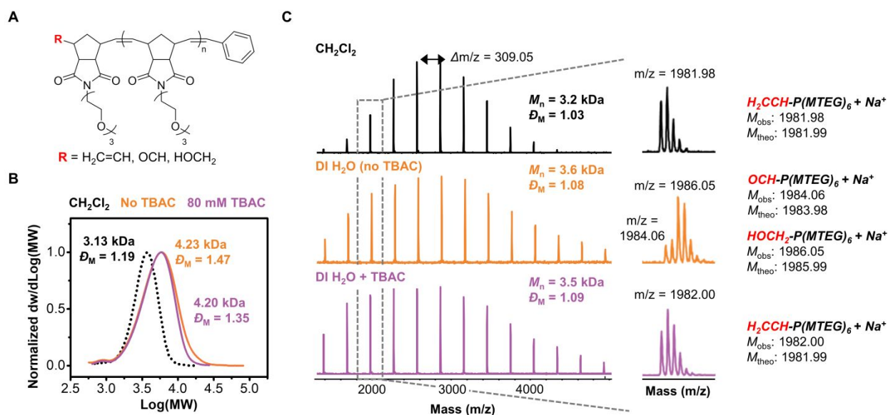
Figure 5. (A) Observed \omega -end groups for P(MTEG) 10 homopolymers synthesized under various conditions. (B) Normalized SEC MW distributions (eluent: THF + 2 v/v% NEt 3 , PS standards) of the P(MTEG) 10 homopolymers. (C) MALDI-ToF mass spectra of the P(MTEG) 10 homopolymers prepared under different conditions. The enlarged regions show the isotopic distributions for the DP P(MTEG) = 6 species highlighted by the dashed square. DCTB was used as the matrix and CF 3 COONa as the cation source.
