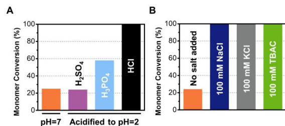
Figure 2. Monomer conversions obtained from additional screening polymerizations of MPEG using G3 to evaluate different acids (A) or salt additives (B), as determined by 1 H NMR spectroscopy in methanol-d 4 .
