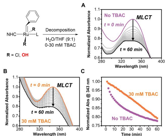
Figure 4. (A) Catalyst decomposition in neutral aqueous media leads to loss of the carbene and a decrease in absorbance of the MLCT band. Shown are the UV-Vis spectra for G3 , collected every 90 s over 1 h, in the absence (A) or presence (B) of 30 mM TBAC. (C) Change in MLCT band absorbance over time depending on incubation conditions.
