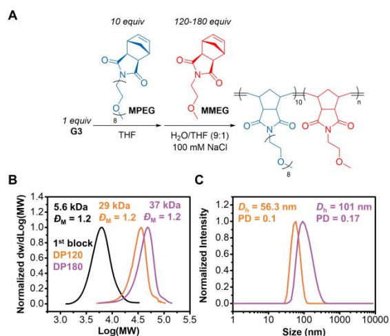
Figure 6. (A) Synthesis of P(MPEG) 10 - b -P(MMEG) n diblock copolymer nano-objects by ROMPISA at neutral pH w/ 100 mM NaCl. (B) Normalized SEC MW distributions (eluent: THF + 2 v/v% NEt 3 , PS standards) of the P(MPEG) 10 macroinitiator and P(MPEG) 10 - b -P(MMEG) n diblock copolymers. (C) Intensity-weighted DLS traces of diblock copolymer nano-objects prepared by aqueous ROMPISA at neutral pH.
