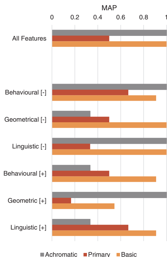
Fig. 5. Class coherence scores when one family of features is excluded [-], and when only one family of features is retained [+], compared to all features (top).
