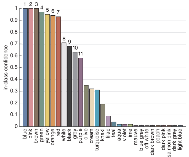
Fig. 3. Class confidences for the basic class. See Fig. 1 for additional notes.
