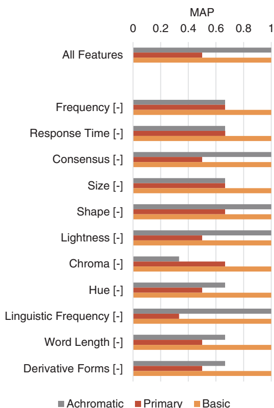
Fig. 4. Class coherence scores when a single feature is excluded [-], compared to when all features are used (top).
