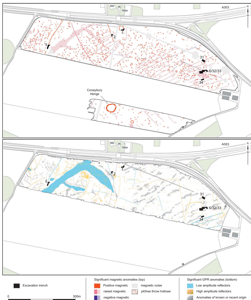
Figure 2. Geophysical survey results (see Linford, Linford, and Payne 2015) and excavation trench locations.
