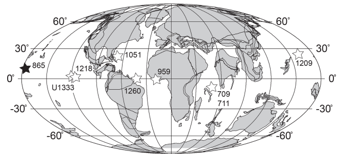
Figure 1. Location map for ODP Site 865 (solid star) and other low-latitude sites discussed in the main text (open stars) on a 40Ma reconstruction. Palaeolatitudes for each site are calculated from van Hinsbergen et al. (2015). Base map generated from http://www.ods.de (last access: 8 June 2018).
