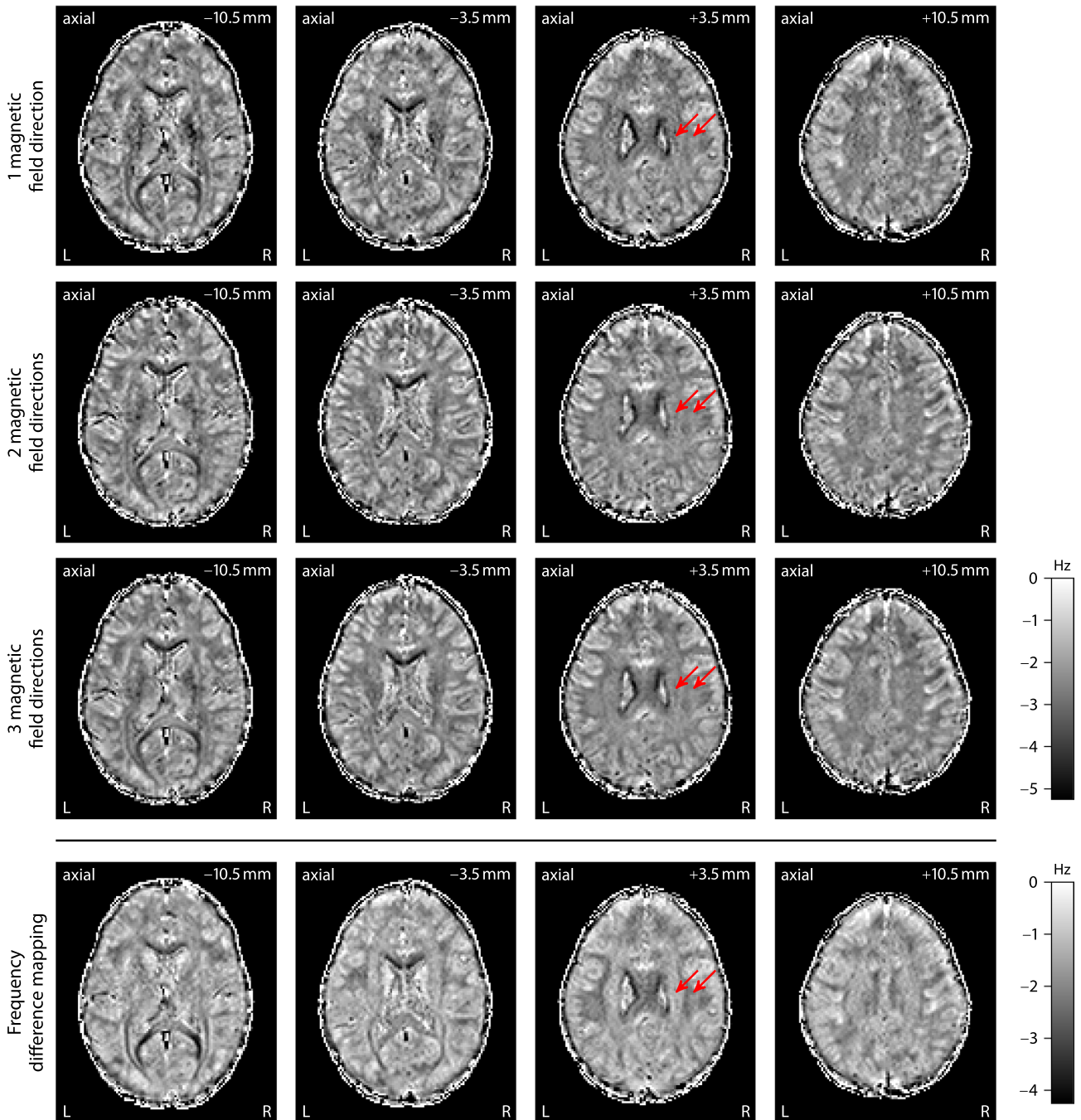
FIGURE 4 Maps of the microscopic frequency shift \omega_{A_{i_0}}(t)/(2\pi) obtained from gradient-echo measurements with different numbers of magnetic field directions at echo time t = 40.5 ms. For comparison, the fourth row shows the macroscopic frequency shift for a single B_0 -direction before factoring out orientational heterogeneity. The 2 arrows point to white matter regions with fiber bundles predominantly running parallel (left) and perpendicular to the external magnetic field in standard head orientation
