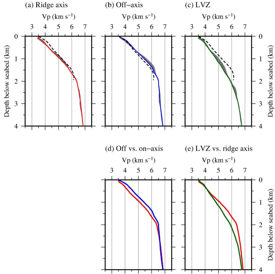
Figure 8. 1-D vertical velocity-depth profiles through the inversion model . a) Velocity-depth profiles at the ridge axis, away from the LVZ ( X=20 km, Y=30 km model space), coinciding with SAP_B. Red line is the inversion model . Grey envelope represents the range of resulting structures from all tested inversion parameterizations. Black dashed line is the Wilson et al. (2019) 2-D OBS inversion velocity-depth structure at the ridge axis. b) Off-axis, 10 km to the south ( X=20 km, Y=40 km; blue line). c) At the location of maximum LVZ amplitude ( X=29 km, Y=31 km; green line). d) Comparison between off- and on-axis velocity-depth profiles through the inversion model . Line colours correspond to the model locations shown in a) & b). e) Comparison between LVZ and ridge axis profiles.
