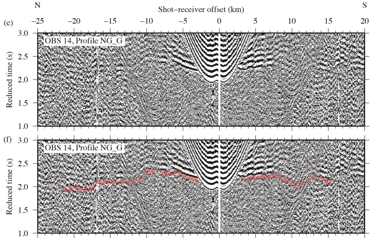
Figure 4. Example OBS hydrophone record sections, displayed using a minimum phase bandpass filter (1-4-88-120 Hz) and a reduction velocity of 6 \text{ km s}^{-1} . a) OBS 07, Profile NG_B, which runs along the ridge axis with b) travel time picks annotated, where bar height corresponds to the assigned pick uncertainty (Table 1). c) & d) OBS 23, Profile NG_E, which is oriented ridge-parallel, off-axis to the south. e) & f) OBS 14, Profile NG_G, oriented across axis and intersecting a) & b).
