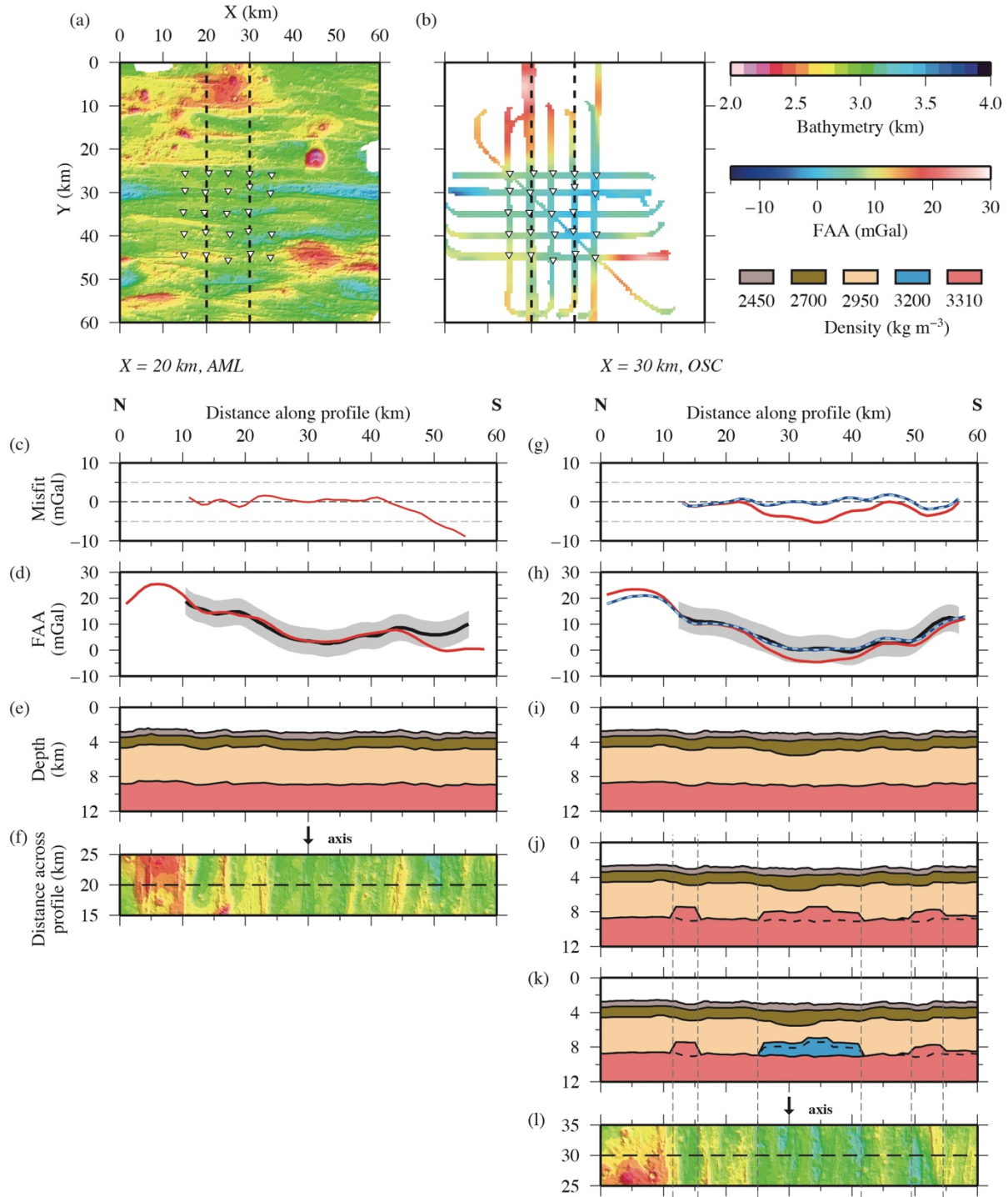
Figure 11. 2-D gravity modelling. a) Ship-acquired swath bathymetry data. Inverted black triangles show OBS locations. Black dashed lines correspond to profile locations shown in c-f) & g-l). b) Cross-over corrected and gridded JC114 ship-acquired FAA. Left: AML gravity modelling ( X=20 km). c) Misfit between observed and modelled FAA. d) Observed (black) and modelled (red) FAA corresponding to the model shown in e). Grey envelope shows the \pm 5 mGal error bound. e) Crustal AML density model , derived using 4.55 and 6.25 \text{km s}^{-1} contours from the inversion model , a constant total thickness crust (6 km), and density from Carlson & Raskin (1984). f) Ship-acquired bathymetry along modelled profile (black dashed line). Black arrow shows the location of ridge axis. Right: OSC gravity modelling ( X=30
