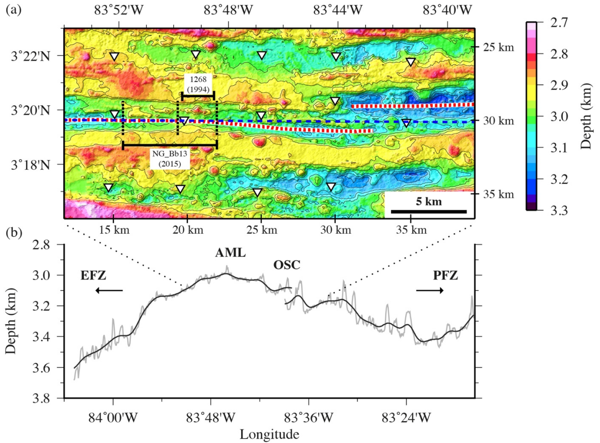
Figure 2. Swath bathymetry of the CRR showing ridge axis structure. a) Ridge axis in the vicinity of the overlapping spreading segment. Red dashed line indicates the location of ridge axis centre line. Blue dashed line is the location of OSCAR MCS Profile NG_Bb13 (Lowell et al., 2020), co-incident with the location of EW9416 Profile 1268 (Buck et al., 1997). Dashed black lines show the longitudes of the ends of the observed AML from these two surveys. Inverted triangles show OBS locations (cf. Fig. 1b ). b) Bathymetry sampled along the ridge axis centre line (light grey), shown with a 3' (~5 km) Gaussian filter applied (dark grey). Dotted black lines show location relative to a). Labelled arrows indicate the directions to and names of bounding fracture zones (cf. Fig. 1a ). OSC and AML locations along the ridge axis are labelled.
