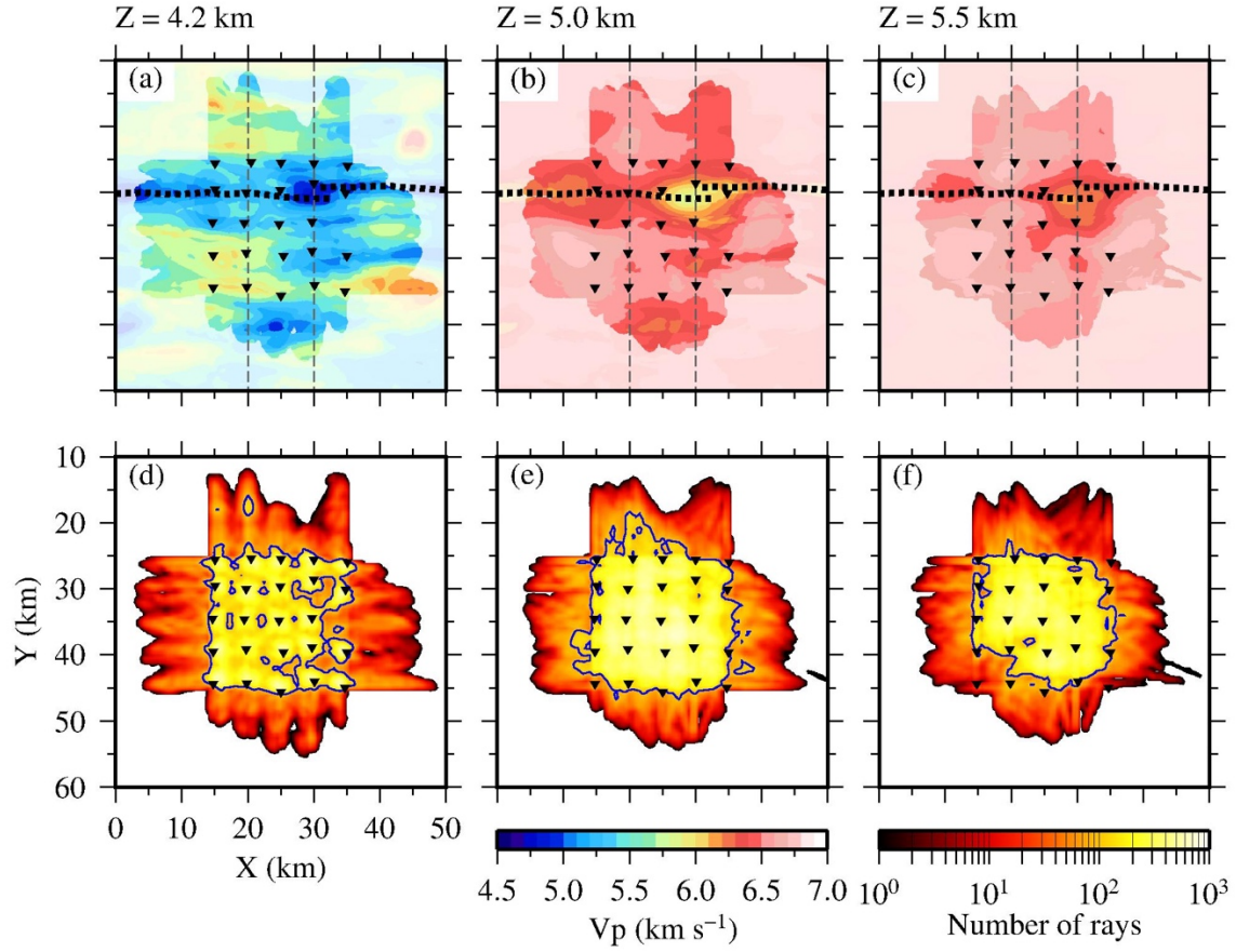
Figure 6. Inversion model derived with 0.5 km lateral and 0.5 km vertical inversion cells. Horizontal (constant model depth) slices at: a) Z=4.2 km ( \sim 1.2 km b.s.f.); b) Z=5.0 km ( \sim 2.0 km b.s.f.), and c) Z=5.5 km ( \sim 2.5 km b.s.f.). Illumination masking shows the extent of model ray coverage and the dotted line shows the centre line of the west and east CRR ridge segments. Inverted black triangles show OBS locations. Dashed grey lines show locations of vertical slices shown in Fig. 5b-d . d-f) Corresponding ray coverage. Blue line delimits inverse cells with more than 100 ray hits.
