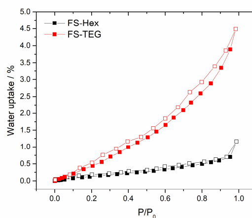
Figure 3. Water vapor isotherms of FS-Hex and FS-TEG at 20.0 °C and up to 23 mbar.
