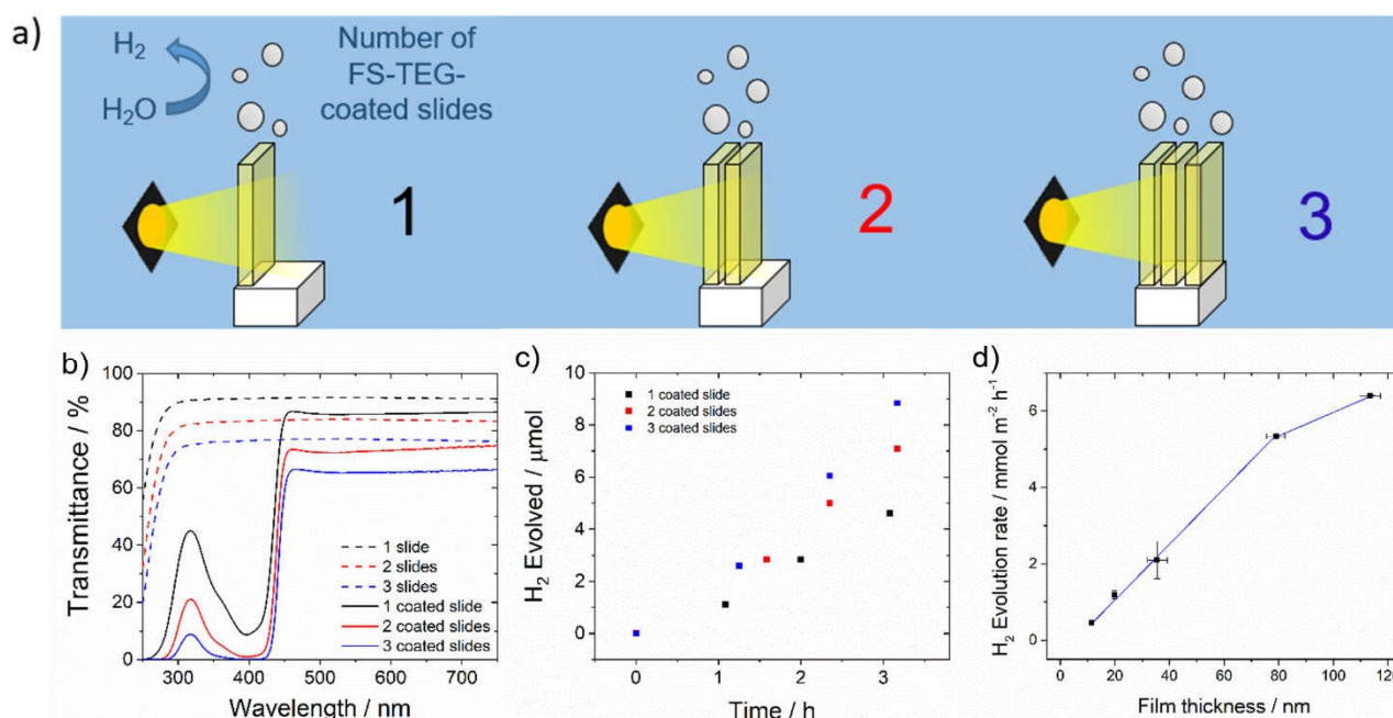
Figure 5. a) Schematic diagram of FS-TEG-coated glass slides stacked in series under the experimental conditions; b) UV-Visible transmittance spectra of slides stacked in series; c) Hydrogen evolved by stacked films in series under visible light; d) Hydrogen evolution rates of FS-TEG films of varying thicknesses. Conditions for c) and d): Spin-coated from chloroform solution onto OTS-functionalized glass slides; 5 vol. % TEA in water, irradiated with visible light ( \lambda > 420 nm filter, 300 W Xe light source).
