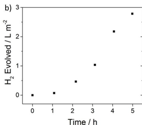
Figure 9. a) Side-view of the photoreactor set-up with reflective panel and polymer-coated glass fibers submerged in 5 vol. % TEA and connected to a hydrogen collection vessel (right) b) Amount of hydrogen evolved over a 5-hour period on a largely overcast day (see supporting video of the experiment).
