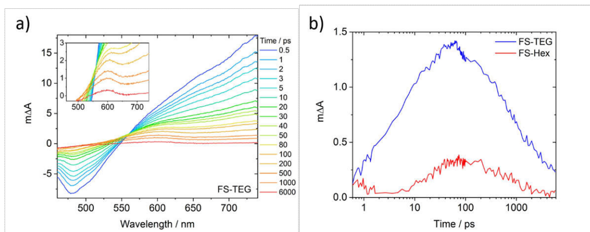
Figure 7. a) fs-TAS spectra of an FS-TEG dispersion in water/methanol/TEA. The color scale is measured in picoseconds after 420 nm excitation. Inset: Magnified spectra highlighting the 600 nm absorption feature; b) Deconvoluted fs-TAS kinetics of the electron, probed at 600 nm, for dispersions of FS-TEG and FS-Hex . These kinetics were calculated by subtracting the shape of the TAS spectrum at 0.5 ps, at which point only excitons have formed, from all subsequent times. Both 0.2 mg mL -1 samples were measured under identical fluences of 87 μm 2 .
