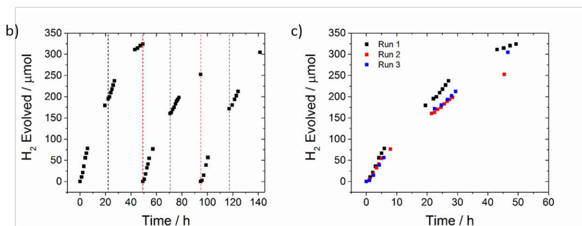
Figure 6. a) Images of free-standing film suspended in 5 vol.% TEA before and after photocatalytic experiment; b) Hydrogen evolution of free-standing film of FS-TEG from a 5 vol.% TEA mixture under \lambda > 420 nm irradiation over a period of 141 hours with intermittent degassing (black dashed lines) and replacement of scavenger mixture (red dashed lines) (300 W Xe light source); c) Direct comparison of hydrogen evolution runs after replacing the scavenger mixture.
