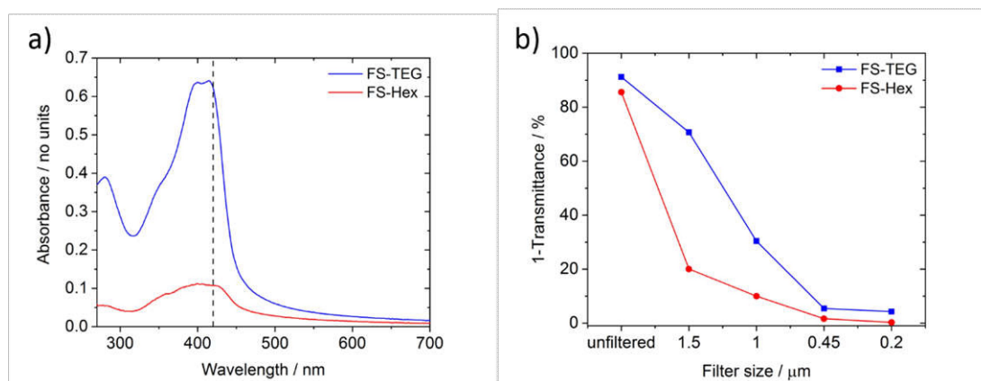
Figure 2. a) Absorption spectra of FS-TEG and FS-Hex dispersions in water/methanol/TEA (1:1:1), filtered from 1 mg mL -1 dispersions using a 1.5 μm filter to reduce scattering. The dashed line is at 420 nm; b) (1-Transmittance) at 420 nm of FS-TEG and FS-Hex samples which have been filtered from 1 mg mL -1 dispersions with Nylon filters of different pore sizes (see also Fig. S-58 for spectra). All polymers were dispersed in water/methanol/TEA and measured in a 1 mm quartz cuvette.
