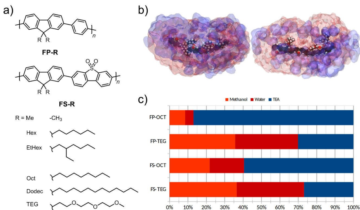
Figure 1. a) Structure of the fluorene co-phenyl (FP-R) and fluorene-co-dibenzo[ b,d ]thiophene sulfone (FS-R) polymer series where R is the alkyl group which is modified as shown; b) Molecular dynamics simulations of FS-Oct and FS-TEG in 1:1:1 water/methanol/TEA. TEA is shown in blue, and the water / methanol phase is shown in pink. In these simulations, FS-TEG draws a substantially higher concentration of water close to the polymer backbone at the expense of TEA; (c) Bar chart showing fraction of volume within a 2 nm radius of the oligomer that is occupied by each component in the liquid medium: methanol (orange), water (red) and TEA (blue).
