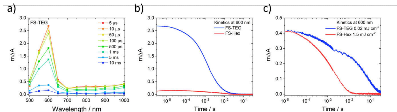
Figure 8. Microsecond transient absorption data taken on 0.02 mg mL -1 water/methanol/TEA FS-TEG and FS-Hex dispersions, excited at 420 nm. a) Spectrum of an FS-TEG dispersion showing the 600 nm feature, assigned to electron polaron absorption, as the only feature; b) Electron kinetics for FS-TEG and FS-Hex dispersions, illuminated with an excitation fluence of 0.92 mJ cm -2 ; c) Electron kinetics for FS-TEG and FS-Hex dispersions, illuminated at different excitation fluences. The FS-Hex sample was first excited at a fluence of 1.5 mJ cm -2 . The incident fluence on the FS-TEG sample was then adjusted to 0.02 mJ cm -2 such that it had a comparable maximum ΔA at 600 nm, indicating a similar electron density.
