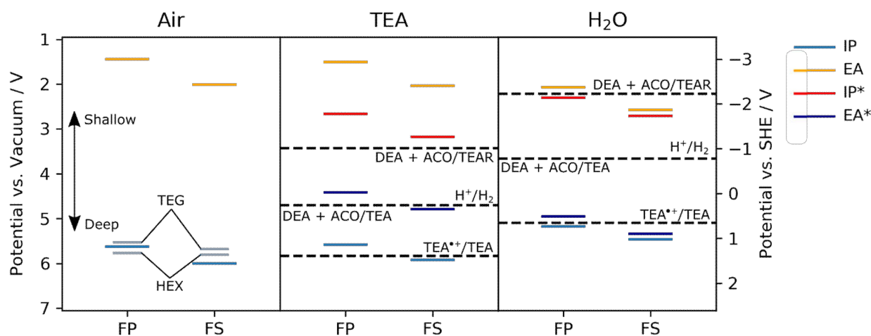
Figure 4. Experimental potentials for FP-TEG , FP-Hex , FS-TEG and FS-Hex films in air (left panel, shorter, light blue lines) and DFT-predicted ground and excited-state ionization potentials and electron affinities of FP-Me and FS-Me in the presence of air (left panel, thicker lines), TEA (central panel) and water (pH ~11, right panel). In the DFT (B3LYP/DZP) 41-44 calculations the polymers are modelled as single strands embedded in a dielectric continuum 45 with a relative dielectric permittivity value of 80.1, 2.38 and 2.0, describing the dielectric screening of charges in the polymer near the surface of the polymer particles by water, TEA or the polymers themselves in the absence of a liquid ( i.e. , air) respectively. Solution potentials have been taken from previous work, 29 where protons in all half-reactions were modelled as adducts with TEA ( i.e. TEA:H + ). TEA 2+ = charged triethylamine radical; DEA = diethylamine; ACO = acetaldehyde; TEAR = neutral triethylamine radical.
