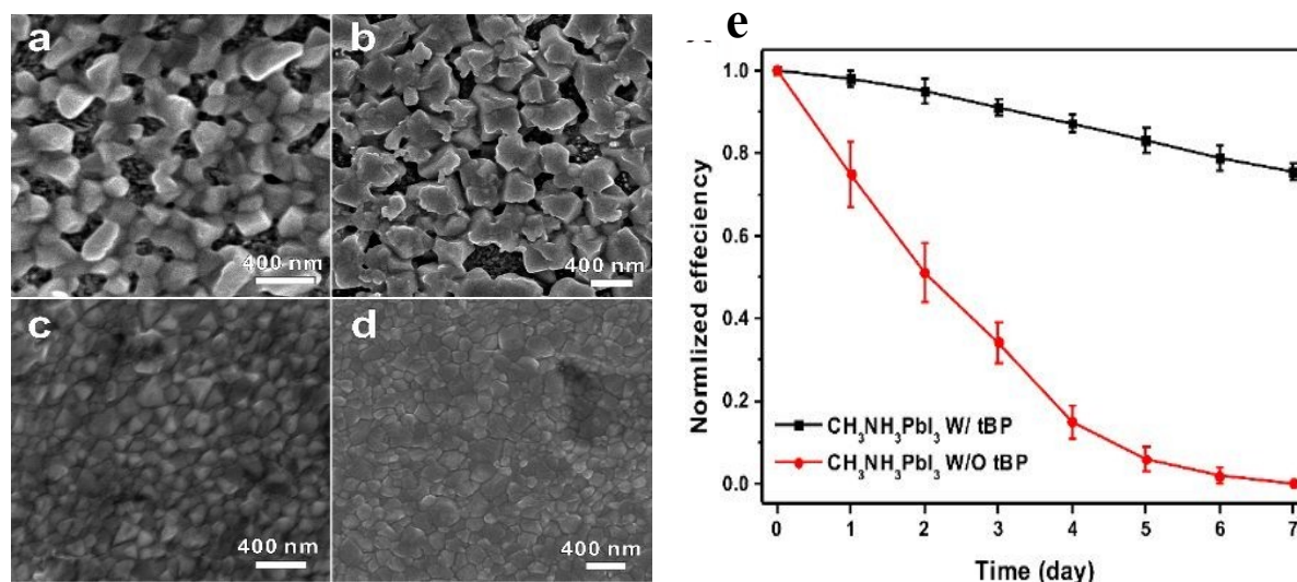
Fig. 5 Scanning electron microscope images of \text{PbI}_2 and \text{MAPbI}_3 thin films (a,b) without tBP additive and (c,d) with tBP additive. (e) Evolution of the power conversion efficiencies of \text{MAPbI}_3 with tBP and \text{MAPbI}_3 without tBP-based solar cells with respect to time. Reproduced by permission ref. 58, Copyright 2017 American Chemical Society.
