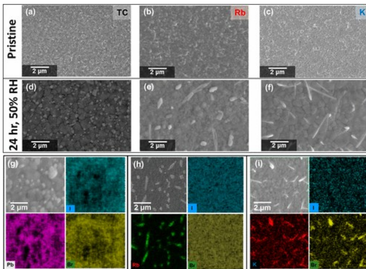
Fig. 11 Scanning electron microscope top-view images of pristine (top row) and with 50% relative humidity, nitrogen over a course of twenty-four hours (second row) (a,d) triple cation, (b,e) Rb-passivated triple cation, and (c,f) K-passivated triple cation perovskite thin films. SEM image with EDX elemental mapping of the same (g) triple cation, (h) Rb-passivated triple cation and (i) K-passivated triple cation perovskite thin films. Reproduced by permission ref. 92, Copyright 2018 American Chemical Society.
