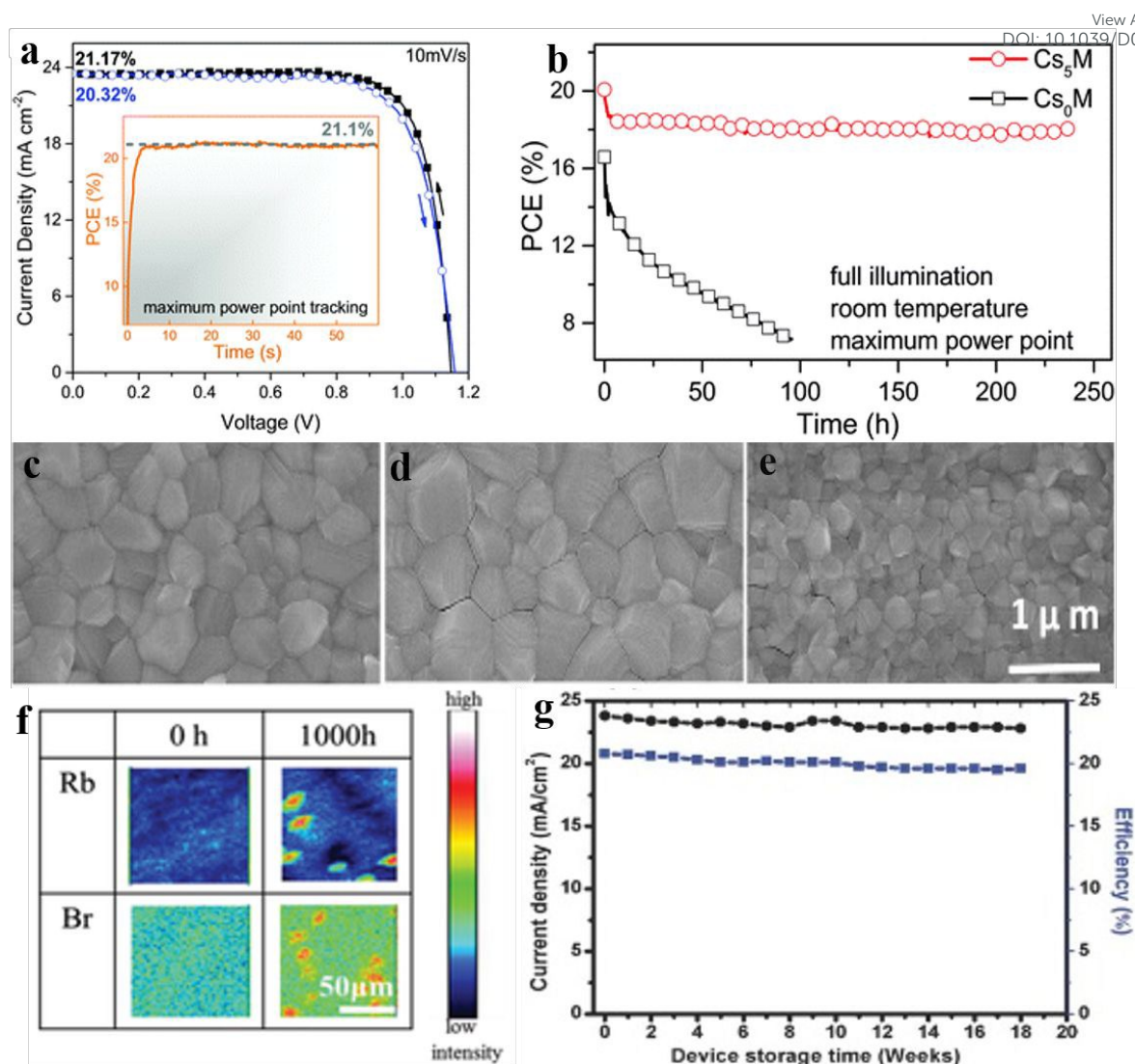
Fig. 10 (a) I-V scan for \text{Cs}_5\text{M} device that shows power conversion efficiency above 21% (b) Change in device efficiency with time up to 250 hours of a high-performance \text{Cs}_5\text{M} and \text{Cs}_0\text{M} devices which kept in \text{N}_2 atmosphere at room temperature with constant illumination and maximum power point tracking. Reproduced by permission ref. 89, Copyright 2016 Royal Society of Chemistry. Top view scanning electron microscope images of perovskite thin films made from (c) \text{Cs}_0 , (d) \text{Cs}_5 , (e) \text{Cs}_{10} . Reproduced by permission ref. 88, Copyright 2017 WILEY-VCH Verlag GmbH & Co. KGaA, Weinheim. (f) Top-view TOF-SIMS elemental mapping of the \text{Rb}_{0.05}\text{Cs}_{0.05}\text{FA}_{0.75}\text{MA}_{0.15}\text{Pb}(\text{I}_{0.83}\text{Br}_{0.17})_3 perovskite thin film before and after thermal stress test at 85 °C for 1000 h. Reproduced by permission ref. 90, Copyright 2019 WILEY-VCH Verlag GmbH & Co. KGaA, Weinheim. (g) Current density and efficiency change with device storage time in weeks. Reproduced by permission ref. 88, Copyright 2017 WILEY-VCH Verlag GmbH & Co. KGaA, Weinheim.
