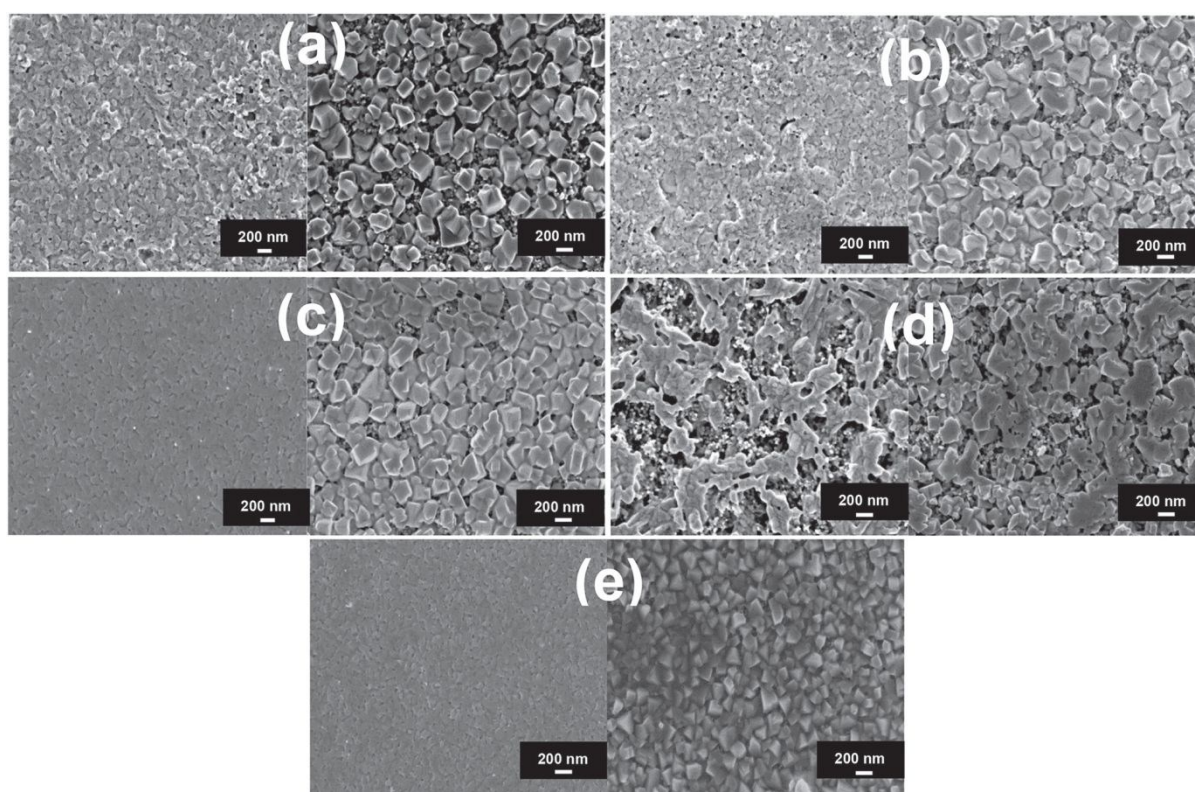
Fig. 6 Top-view SEM images of \text{PbI}_2 (left side) and \text{CH}_3\text{NH}_3\text{PbI}_3 (right side) structures: a) pristine, b) CuBr, c) CuI, d) NaI, and e) AgI based perovskite samples deposited on a mesoporous \text{TiO}_2 - coated FTO. Reproduced by permission ref. 69, Copyright 2016 WILEY-VCH Verlag GmbH & Co. KGaA, Weinheim.
