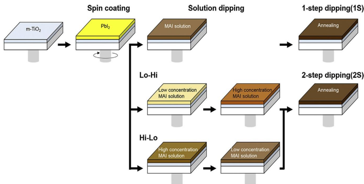
Fig. 18 Schematic diagram of the fabrication process of CH 3 NH 3 PbI 3 perovskite films. Here 1S means one-step MAI dipping as conventional sequential deposition process and 2S means two-step MAI dipping by changing MAI concentration as Lo-Hi and Hi-Lo. Reproduced by permission ref. 126, Copyright 2016 Elsevier B.V.
