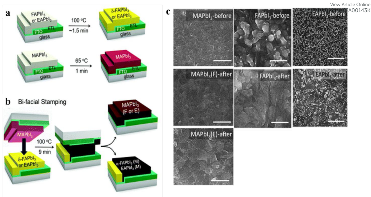
Fig. 24 Schematic diagram of the stamping technique includes two steps. (a) pre-annealing () and (b) the bifacial stamping technique. (c) Plane-view scanning electron microscopy images of MAPbI 3 -before, MAPbI 3 (F)-after, MAPbI 3 (E)-after, FAPbI 3 -before, FAPbI 3 (M)-after, EAPbI 3 -before and EAPbI 3 -after. Scale bars are 1 \mu m. Reproduced by permission ref. 160, Copyright 2019 Royal Society of Chemistry.
