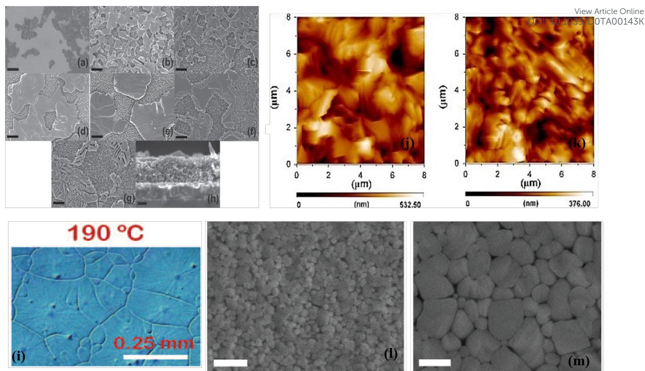
Fig. 2 Scanning electron microscope images of m-TiO 2 films with deposited perovskite solution heat-treated at different temperature a) 60°C, b) 80°C, c) 100°C, d) 120°C, e) 150°C, f) 175°C and g) 200°C. h) Cross-sectional SEM image of the sample annealed at 150°C. Black scale bars correspond to a) 5 μm, b-g) 1 μm, and h) 200 nm. Reproduced by permission ref. 46, Copyright 2014 WILEY-VCH Verlag GmbH & Co. KGaA, Weinheim. Optical micrograph of CH 3 NH 3 PbI 3-x Cl x perovskite thin film (i). Reproduced by permission ref. 47, Copyright 2015 American Association for the Advancement of Science. Atomic force microscopy images of perovskite thin films annealed with the one-step method (j), multi-step method (k). Reproduced by permission ref. 43, Copyright 2015 Elsevier B.V. Scanning electron microscope image of an unannealed hot-cast film (l) and an annealed hot-cast film (m), showing that the perovskite crystals grow during annealing. Reproduced by permission ref. 45, Copyright 2016 WILEY-VCH Verlag GmbH & Co. KGaA, Weinheim.
