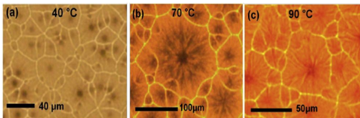
Fig. 4 Optical microscopic images of perovskite thin films with different perovskite solution temperatures of (a) 40^\circ\text{C} , (b) 70^\circ\text{C} and (c) 90^\circ\text{C} . Reproduced by permission ref. 53, Copyright 2016 Elsevier B.V.
