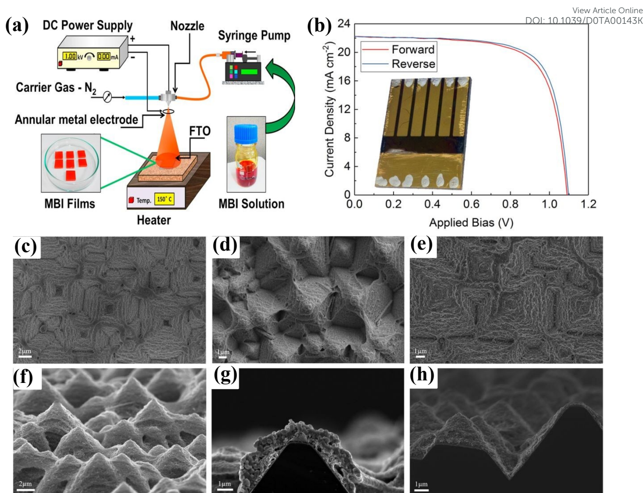
Fig. 26 (a) Schematic illustration of spray coating process with the application of DC voltage used in the fabrication of lead free \text{MA}_3\text{Bi}_2\text{I}_9 perovskite thin films. Reproduced by permission ref. 170, Copyright 2019 International Solar Energy Society. (b) J-V characteristics for the spraycast triple-cation PSC showing 17.8% efficiency in reverse scan. The device photograph is shown in inset. Reproduced by permission ref. 167, Copyright 2018 American Chemical Society. Top-view and cross-section SEM images of the spray-coated films onto the textured silicon bottom cell. (c,f) \text{PbI}_2 NC ink, (d,g) \text{MAPbI}_3 perovskite, and (e,h) \text{CsFAMAPbI}_{3-x}\text{Br}_x mixed perovskite films after spray conversion. Reproduced by permission ref. 169, Copyright 2020 WILEY-VCH Verlag GmbH & Co. KGaA, Weinheim.
