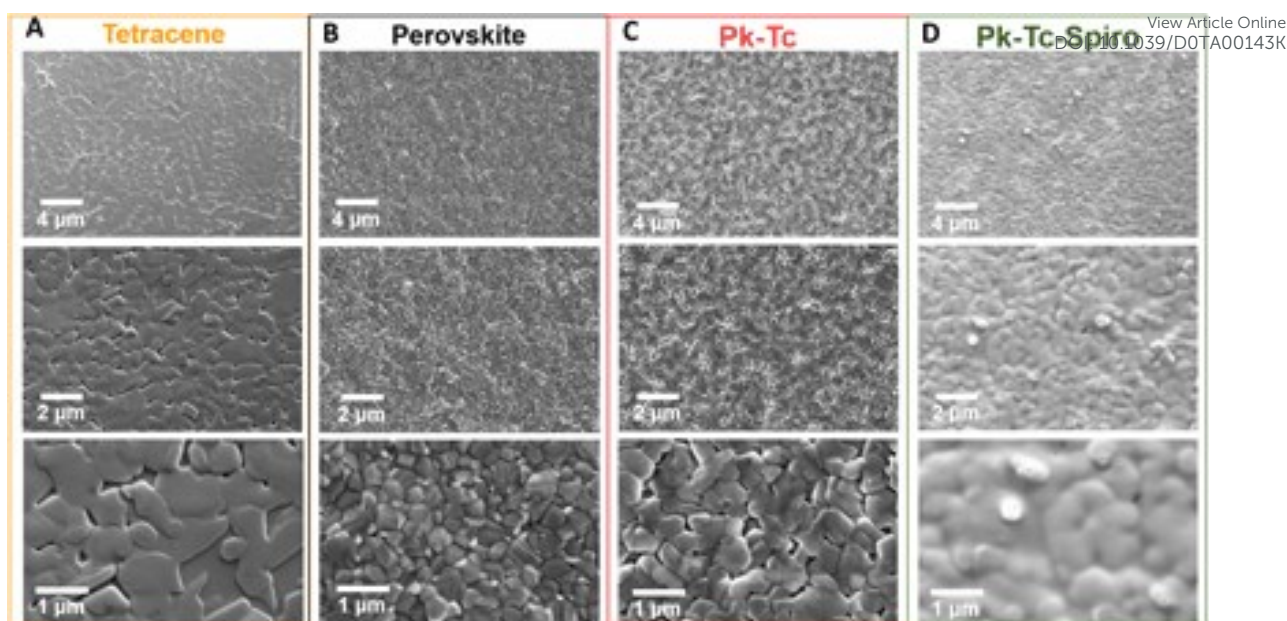
Fig. 13 Top-view scanning electron microscopy of (A) tetracene (Tc) single layer, (B) perovskite (Pk), (C) perovskite-tetracene (Pk-Tc), and (D) perovskite-tetracene-Spiro (Pk-Tc-Spiro) films at three different magnifications. Reproduced by permission ref. 101, Copyright 2018 American Association for the Advancement of Science.
