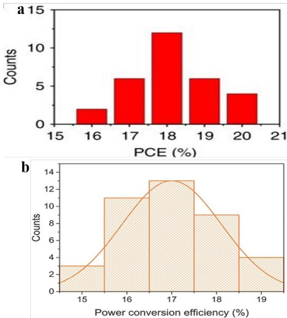
Fig. 22 (a) Histogram of perovskite solar cell efficiencies based on MAPbI 3 : F4TCNQ films (with 0.03 wt% F4TCNQ). Reproduced by permission ref. 145, Copyright 2018 Springer Nature. (b) Histogram of 40 devices based on MA 0.6 FA 0.38 Cs 0.02 PbI 2.975 Br 0.025 : 5 mol% MACl perovskite. Reproduced by permission ref. 146, Copyright 2017 WILEY-VCH Verlag GmbH & Co. KGaA, Weinheim.
