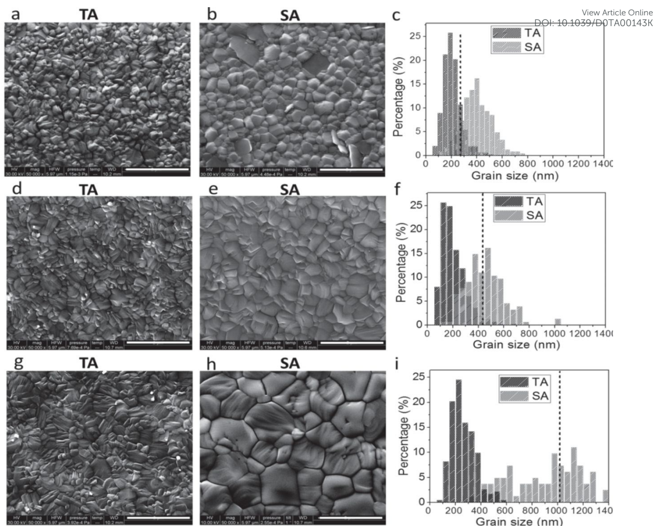
Fig. 15 Scanning electron microscope images of the thermally annealed (TA) perovskite films with thicknesses of 250 nm (a), 430 nm (d), and 1015 nm (g), and solvent-annealed (SA) perovskite films with thickness of 250 nm (b), 430 nm (e) and 1015 nm (h); the scale bars in the SEM micrographs are 2 \mu\text{m} . c,f, i) Grain-size distributions of the SEM images to the left. Reproduced by permission ref. 23, Copyright 2014 WILEY-VCH Verlag GmbH & Co. KGaA, Weinheim.
