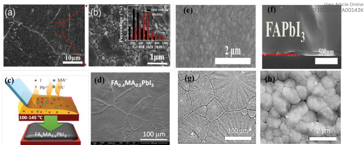
Fig. 21 (a) Scanning electron microscope images of doctor-bladed \text{CH}_3\text{NH}_3\text{PbI}_3 film fabricated at 130^\circ\text{C} . (b) Scanning electron microscope images of the selected area in (a). The grain size distribution of \text{CH}_3\text{NH}_3\text{PbI}_3 films is shown in the inset. The red color is for the doctor-bladed and black color is for spin-coated films. Reproduced by permission ref. 142, Copyright 2017 Elsevier B.V. (c) Diagram of the doctor-blade coating for the fabrication of mixed cation perovskite film. (d) SEM images of \text{FA}_{0.4}\text{MA}_{0.6}\text{PbI}_3 perovskite films fabricated by doctor-blade technique. Reproduced by permission ref. 143, Copyright 2016 WILEY-VCH Verlag GmbH & Co. KGaA, Weinheim. (e) SEM surface image and (f) cross-sectional SEM image of \alpha - \text{FAPbI}_3 films fabricated via doctor-blading. Reproduced by permission ref. 144, Copyright 2017 Elsevier B.V. SEM images of bladed and doped \text{CH}_3\text{NH}_3\text{PbI}_3 perovskite film (g) Low magnification and (h) high magnification. Reproduced by permission ref. 145, Copyright 2018 Springer Nature.
