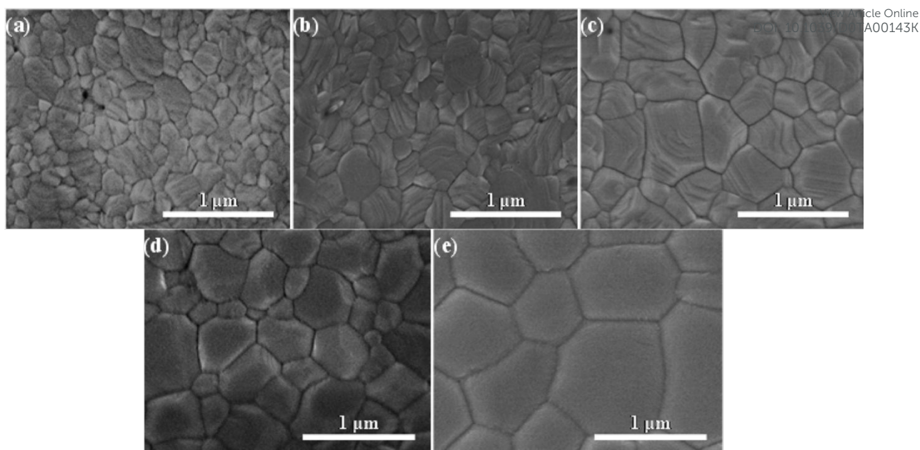
Fig. 17 Surface SEM images of perovskite films on ITO-coated substrate after annealing under different atmospheric conditions: (a) N 2 , (b) H 2 O, (c) GBL, (d) DMF, (e) DMSO. Reproduced by permission ref. 116, Copyright 2015 American Chemical Society.
