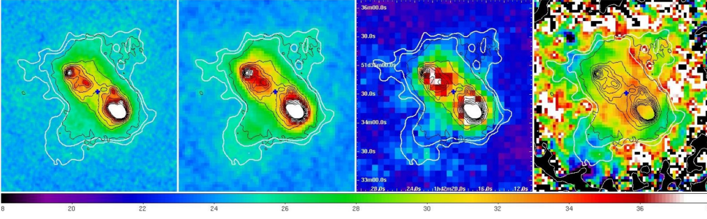
Figure 2. NGC 650, from left to right: PACS 70 and 160 \mu\text{m} , SPIRE 250 \mu\text{m} , and a temperature map. The blue cross marks the central star. The contours were generated the same way as in Fig. 1. The bar on the bottom shows the temperature scale.
