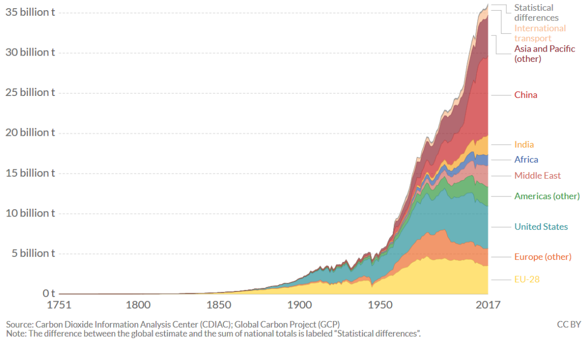
Figure 1: Global CO 2 emissions, which need to become zero by 2050, are still accelerating.
