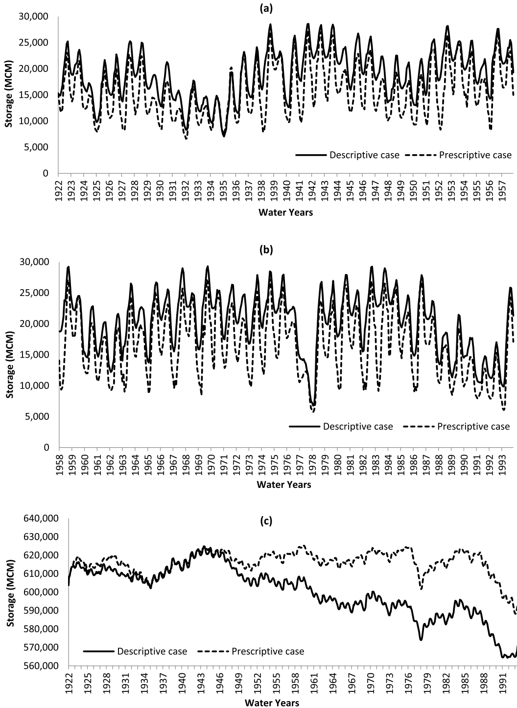
Fig. 8. Comparison of the historical simulation and the optimized model for: a) surface reservoirs over 1922–57; b) surface reservoirs over 1958–93; and c) groundwater over 1922–93.
