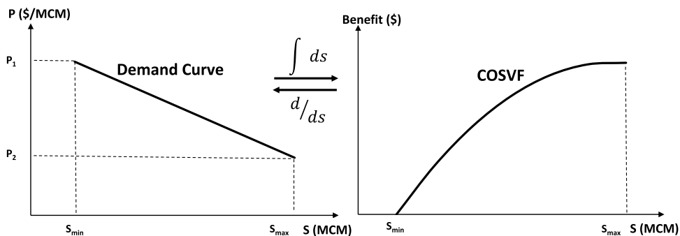
Fig. 1. Relation between demand curve and benefit function of a surface reservoir, in the case of a linear demand function.
