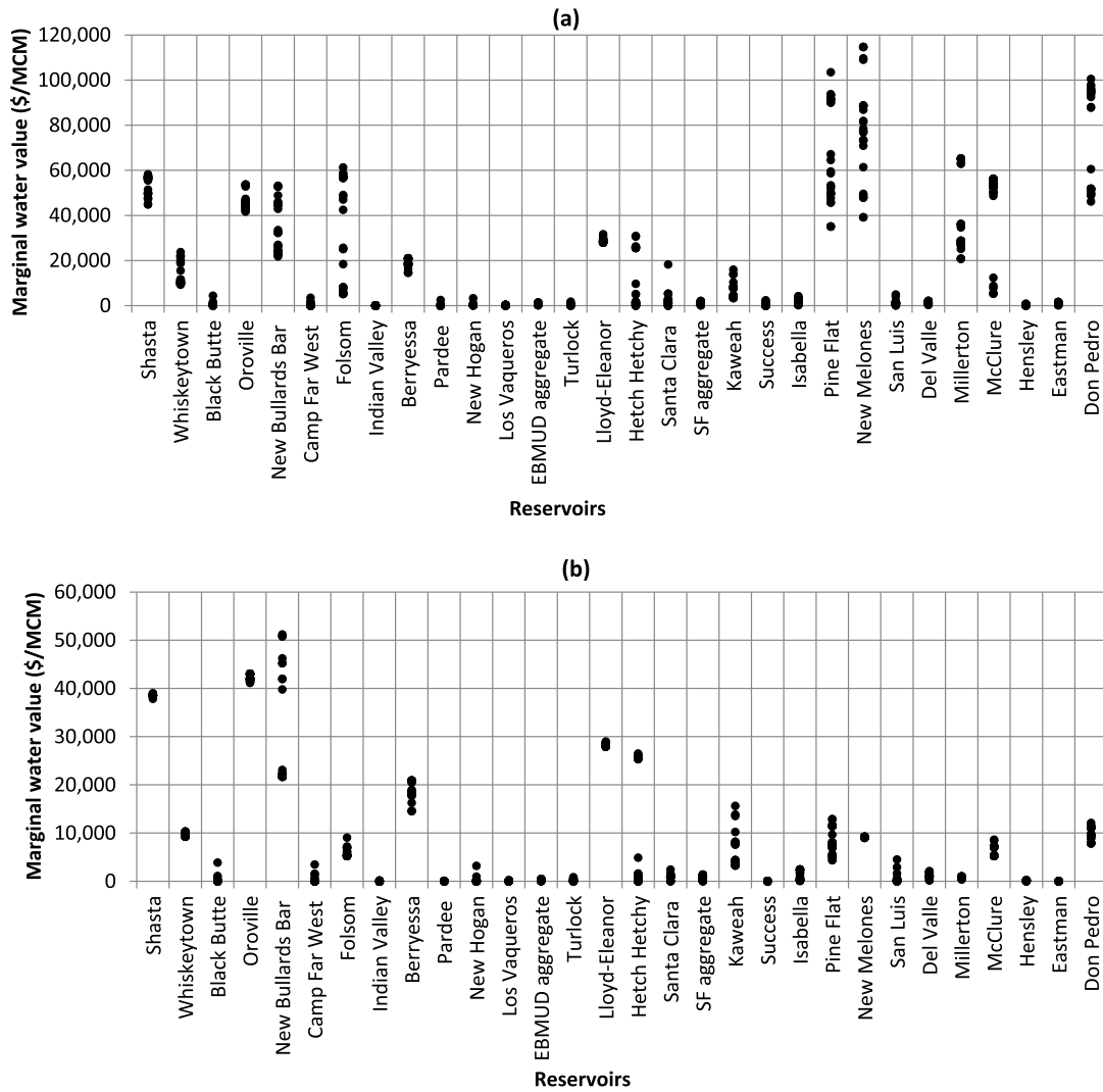
Fig. 5. Dispersion of descriptive marginal water value solutions from zone of concentration at: a) dead storage, and b) full storage.
