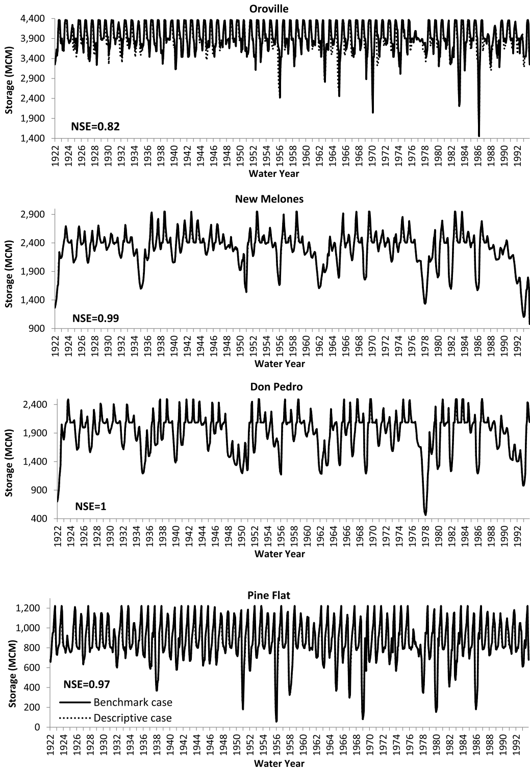
Fig. 4. Comparison of the calibrated storage trajectories of major reservoirs to the benchmark values.
