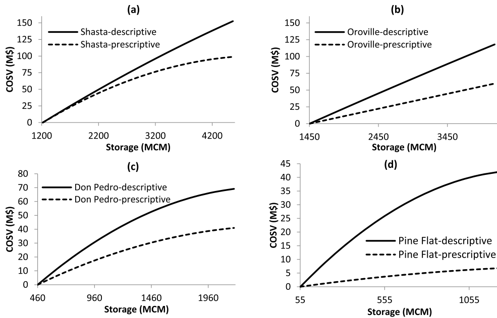
Fig. 7. Comparison of the representative solution in descriptive and normative valuation, COSV of reservoirs in (a) Shasta, (b) Oroville, (c) Don Pedro, and (d) Pine Flat.
