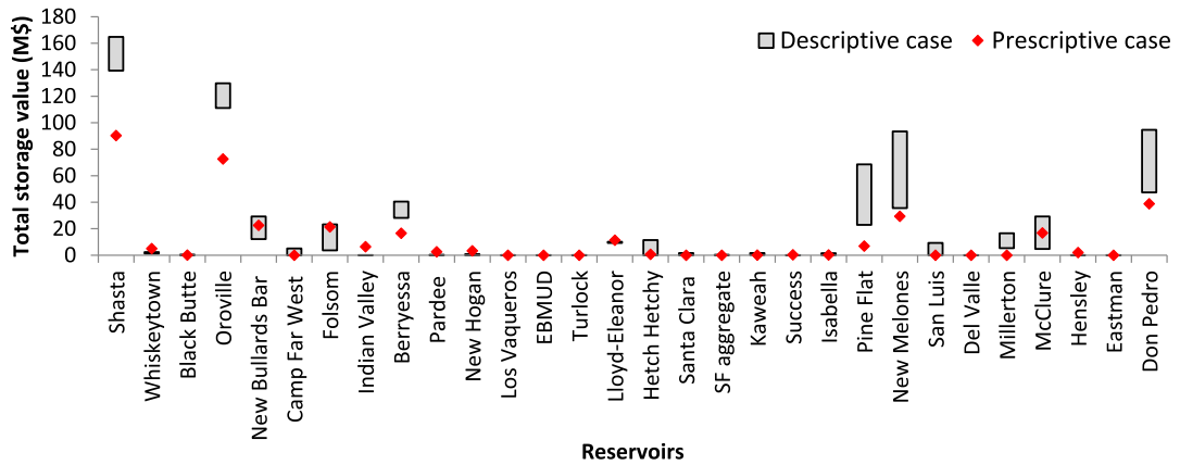
Fig. 6. Distribution of the total storage value from the solution points of the zone of concentration. Red points show the maximum COSVF of the prescriptive solution.
