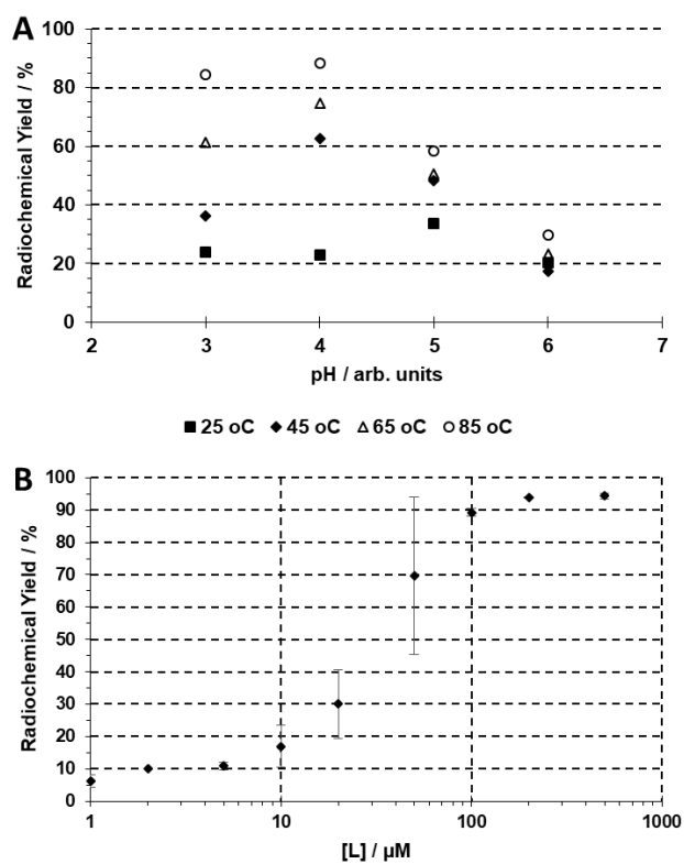
Figure 3. Radiolabelling of L_1 with ^{68}\text{Ga} . A) Effect of pH and temperature on radiolabelling. [L_1] = 100 \mu\text{M} , t = 15 minutes, l = 0.1 \text{ M NH}_4\text{OAc} . B) Effect of concentration on radiolabelling. pH = 4 , T = 95 \text{ }^\circ\text{C} , t = 15 minutes, l = 0.1 \text{ M NH}_4\text{OAc} .
