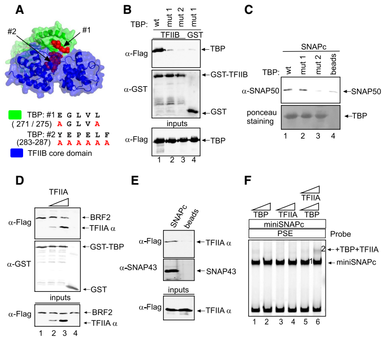
Figure 5. The SNAPc- and TFIIB-interacting surfaces of TBP partially overlap, and TFIIB prevents association of BRF2 with SNAPc and binds to SNAPc cooperatively with TBP. (A) Complex of the TBP and TFIIB core domains (PDB ID: 1c9b), with the two patches of TBP residues mutated to alanines indicated in red, and the alanine substitutions shown at the right. (B) Wild-type or mutant TBPs, as indicated above the lanes, were mixed with GST-TFIIB (lanes 1–3) or just GST (lane 4) attached to beads, and bound proteins were detected by immunoblotting with the antibodies indicated at the left. The bottom panel shows wild-type and mutant TBP inputs. (C) As in B, but SNAPc was mixed with TBP wild type or mutant immobilized on beads or just beads, as indicated above the lanes, and the bottom panel shows wild-type or mutant TBP bound to beads as detected by Ponceau staining. (D) As in B, but BRF2 and TFIIA, as indicated above the lanes, were mixed with GST-TBP (lanes 1–3) or just GST (lane 4). The bottom panel shows BRF2 and TFIIA (as detected by its TFIIA \alpha subunit) inputs. (E) A PSE-containing biotinylated DNA probe was combined with SNAPc and TFIIA (lane 1) or just TFIIA (lane 2). DNA-associated protein complexes were collected on streptavidin beads, and bound proteins were detected by immunoblots with the antibodies indicated at the left. The bottom panel shows input protein.
