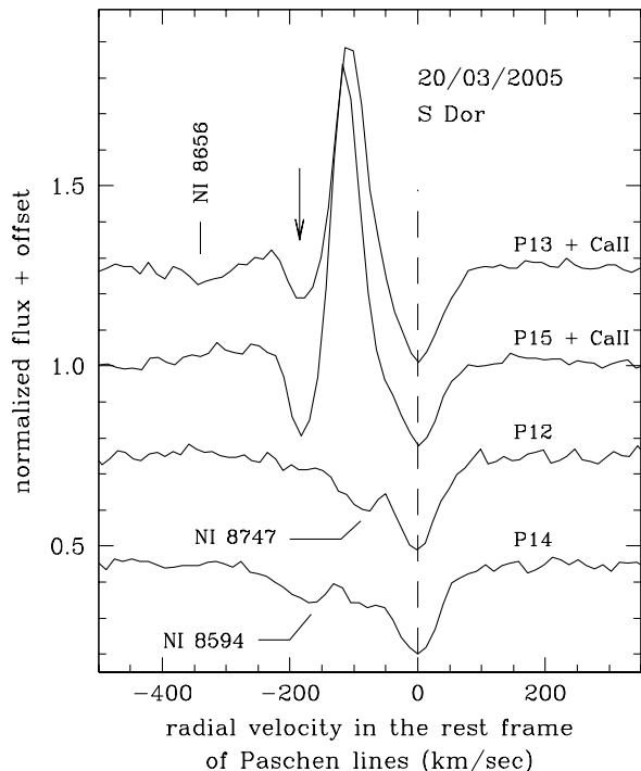
Fig. 5. Expanded view of the S Doradus spectrum of Figure 1 near the Paschen 12 + NI 8747, Paschen 13 + CaII 8662, and Paschen 15 + CaII 8542 features. The arrow points to the absorption component of the CaII P-Cygni profiles.
