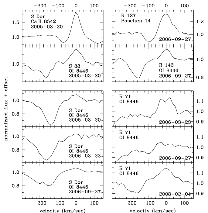
Fig. 4. Sample of P-Cygni profiles of LBVs from RAVE spectra.
