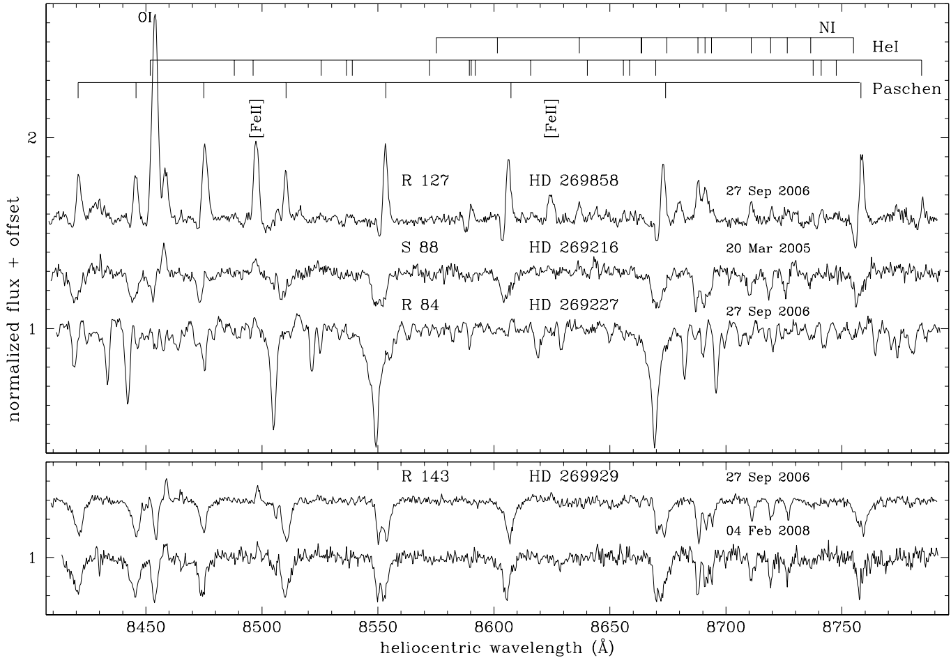
Fig. 3. RAVE spectra of R 127, S 88, R 84, and R 143.
