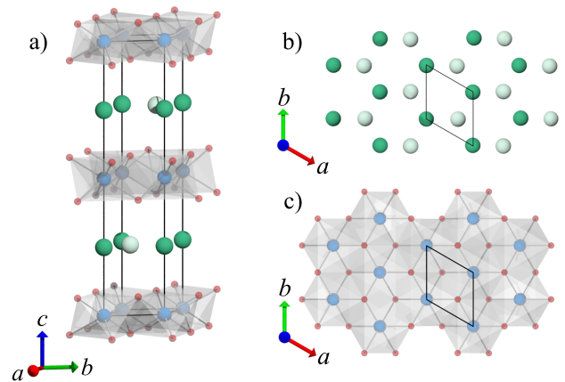
FIG. 3. The Type I crystal structure of K_xIr_{1-x/4}O_2 ( x = 0.61 ) supporting triangular Ir layers. a) A single unit cell drawn with black lines, b) the K1 (dark green spheres) and K2 (light green spheres) potassium triangular substructures at z = 1/4 , and c) the Ir_{1-x/4}O_2 triangular layer at z = 0 . Iridium and oxygen ions are shown as blue and red spheres, respectively, and IrO_6 octahedra are shaded grey.
