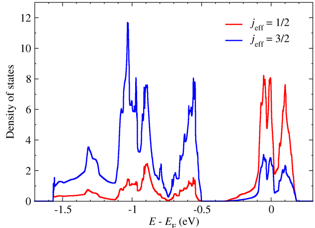
FIG. 6. Density of states (DOS) for theoretical \text{K}_2\text{IrO}_3 obtained within GGA+SOC projected onto the j_{\text{eff}} basis.
