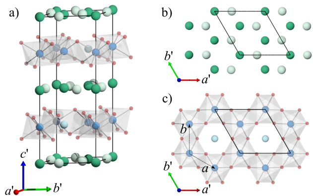
FIG. 4. The Type II crystal structure of \text{K}_x\text{Ir}_{1-x/4}\text{O}_2 ( x = 0.85 ) supporting honeycomb Ir layers. a) A single unit cell drawn with black lines, b) the K11, K12 (dark green spheres) and K2 (light green spheres) potassium triangular substructures at z = 0 , and c) the \text{IrO}_2 triangular layer at z = 1/4 . Iridium, partially occupied iridium, and oxygen ions are shown as blue, light blue, and red spheres, respectively, and fully occupied \text{IrO}_6 octahedra are shaded grey. For comparison, the lattice basis vectors of the triangular structure are drawn as faint dotted lines.
