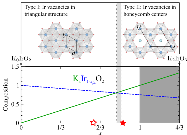
FIG. 1. Proposed conceptual phase diagram for K_x \text{Ir}_{1-x/4} \text{O}_2 as a function of the potassium composition x . The top diagrams indicate the two structural models for the iridium-oxide layer discussed in the text: Type I, where the Ir vacancies are uniformly distributed on all sites (blue spheres) of a triangular layer, and Type II, where Ir vacancies only occupy the centres (light blue spheres) of a honeycomb structure of filled Ir sites. The vertical grey bar at x_c = 0.82 \pm 0.02 indicates the DFT predicted boundary between the two structure types. In the bottom diagram, the blue dashed and solid green lines show the variation of the iridium and potassium compositions, respectively. The solid grey shaded region for x \in [1, 4/3] indicates potentially unphysical bonding of potassium in the honeycomb centres. The two representative compositions discussed in detail in the main text are indicated by open and filled red stars on the horizontal bottom axis.
