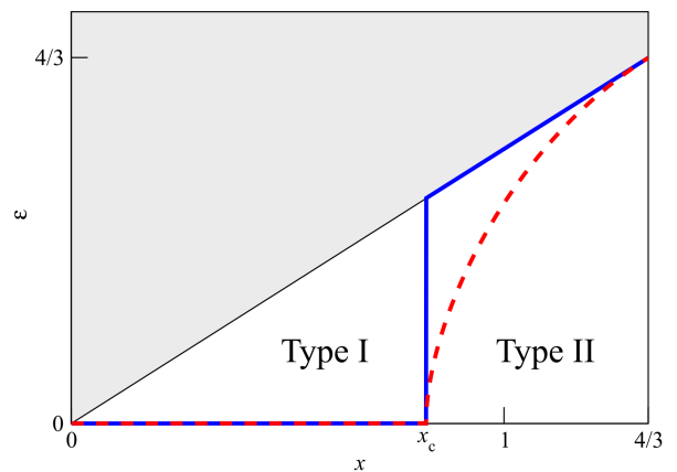
FIG. 7. Schematic representation of the order parameter, \epsilon , for iridium vacancy ordering, as a function of potassium concentration, x , for two generic cases (blue solid and red dashed lines). Below the phase transition at x_c , iridium vacancies are uniformly distributed on the triangular structure ( \epsilon = 0 ). Above x_c , \epsilon may jump to its maximum allowed value for a given x (solid blue line, \epsilon = x ), corresponding to a fully occupied honeycomb structure with partially occupied honeycomb centres. The red dashed line illustrates another possible scenario where \epsilon increases gradually corresponding to a structure with a finite but not complete preferential vacancy occupation at honeycomb centres. The solid black line passing through the origin ( \epsilon = x ) marks the limit above which (grey shaded region) iridium site occupations are unphysical ( > 1 ).
