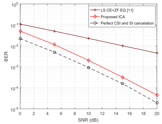
Fig. 3. BER performance of the propose ICA assisted FD relay system and the existing method [11] at \gamma_R^{\text{IPSI}}=0 dB.
