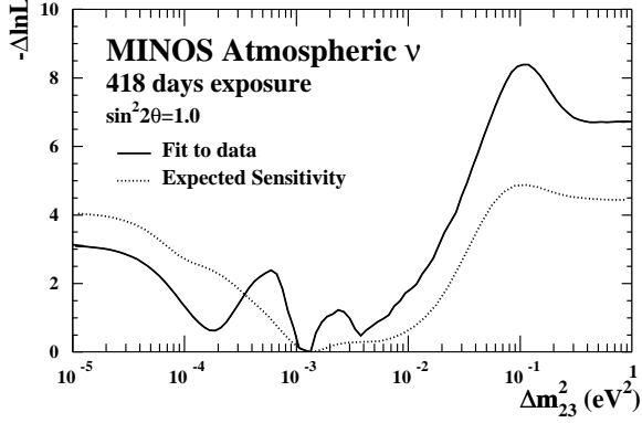
FIG. 14: The \Delta\mathcal{L} curve as a function of \Delta m_{23}^2 for the case of maximal mixing. The dotted curve shows the expected sensitivity which is the average likelihood curve obtained from 10000 Monte Carlo experiments.
