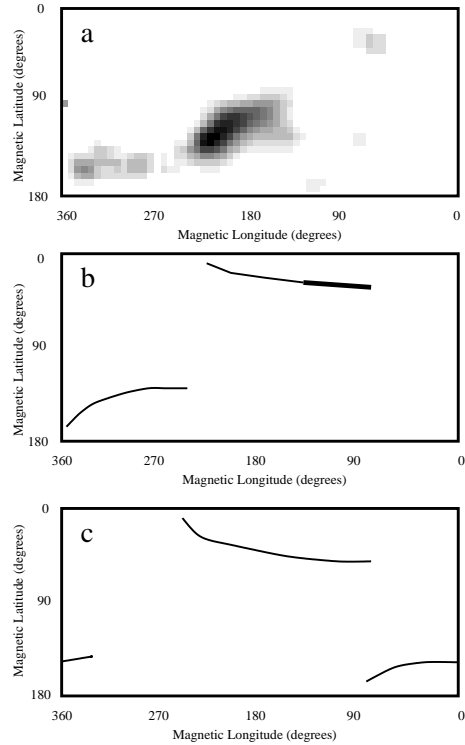
Figure 4. A comparison between: a. The optimised image solution. b. The model prediction in Ramsay et al. (1996) c. The model prediction of Bailey et al. (1995).
