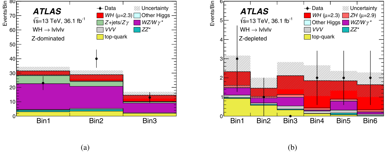
Fig. 6. Post-fit BDT-score distributions (a) in the WH Z-dominated SR and (b) for the two-dimensional grid in BDT_{\tilde{t}\bar{t}} and BDT_{WZ} in the WH Z-depleted SR. The shaded band includes statistical and systematic uncertainties on both signal and background as estimated by the fit.
