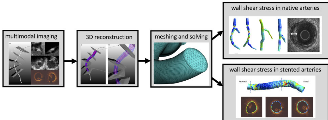
Take home figure Wall shear stress in coronary arteries from imaging to modelling.
