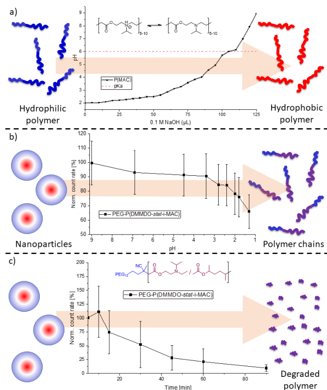
Figure 4: a) P( i -MAC) showed pH sensitive behaviour at a pH of 6.0. At this pH the hydrophilic protonated version (blue) becomes hydrophobic (red). b) The nanoparticles from PEG-P(DMMDO- stat - i -MAC) disassembled into single polymer chains upon acidification from a pH of 4 and below. c) The same nanoparticles were degraded upon the addition of esterase (porcine liver) as shown by the decay of the count rate in DLS.
