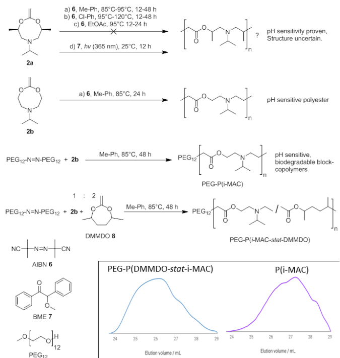
Figure 3: i -DMMAC 2a did not polymerise under various conditions, using different solvents, temperatures and AIBN 6 as an initiator. A polymerisation in bulk using UV-activated polymerisation with BME 7 led to a pH sensitive material. i -MAC 2b yielded a polymer using classic free radical polymerisation with AIBN 6 and was then transformed into a block-copolymer with a PEG-based macroinitiator by itself and also in a 1:2 mix with DMMDO
