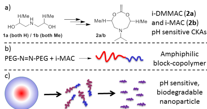
Figure 1: a) The diols 1 containing an amine are transformed into pH sensitive CKAs 2 by ring closure and functional group transformations. b) Polymerising the CKAs with a poly(ethylene glycol) (PEG) based macroinitiator yields amphiphilic block-copolymers, which can then self-assemble into nanoparticles. c) These nanoparticles can disassemble upon acidification (protonation of the amines) or on adding esterase, triggering biodegradation.
