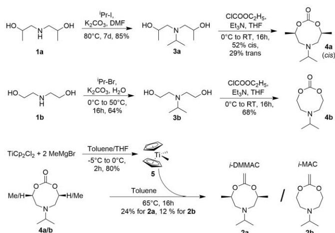
Figure 2: Amino-diols were iso -propylated to give the intermediate diols 3a and 3b . Using ethyl chloroformate, the rings were closed to yield the respective carbonates 4a and 4b . Using freshly prepared Petasis reagent ( 5 ), the carbonates were transformed into the CKAs 2a and 2b .
