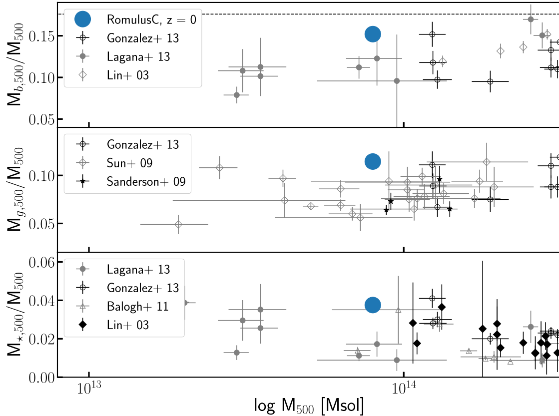
Figure 3. The baryon content of clusters. The total baryon fraction (top), hot gas fraction (middle), and stellar fraction (bottom) by mass in both observed clusters (Lin, Mohr & Stanford 2003; Sanderson, O’Sullivan & Ponman 2009; Sun et al. 2009; Balogh et al. 2011; Gonzalez et al. 2013; Laganá et al. 2013) and ROMULUSC (blue points). All mass fractions for ROMULUSC are within a factor of two of the mean observations at similar masses and within the scatter. We only show z = 0 values for ROMULUSC, but confirm that there is negligible evolution in this respect from z = 0.3 . All observations are for local (redshift below \sim 0.1 ) clusters, though the Laganá et al. (2013) data extend out to higher redshifts.
