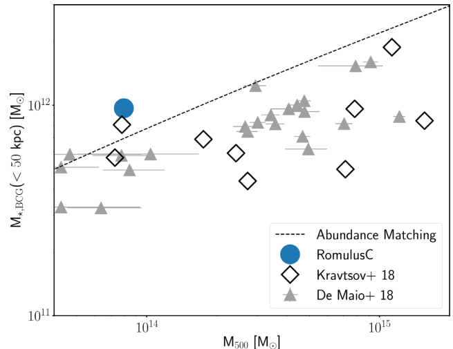
Figure 8. Stellar mass halo mass relation. The relationship between the mass of the central BCG and M_{500} for ROMULUSC (blue point) as well as recent observations from Kravtsov, Vikhlinin & Meshcheryakov (2018) and DeMaio et al. (2018) (black diamonds and grey triangles). Following the observations we compare with here, we consider the stellar mass within 50 kpc from halo centre. Again, we do not plot the z = 0.3 values because there is negligible change from z = 0 . The BCG in ROMULUSC is within a factor of \sim 2 of the median observed BCG stellar mass and matches well with abundance matching results derived from updated luminosity functions (Kravtsov et al. 2018).
