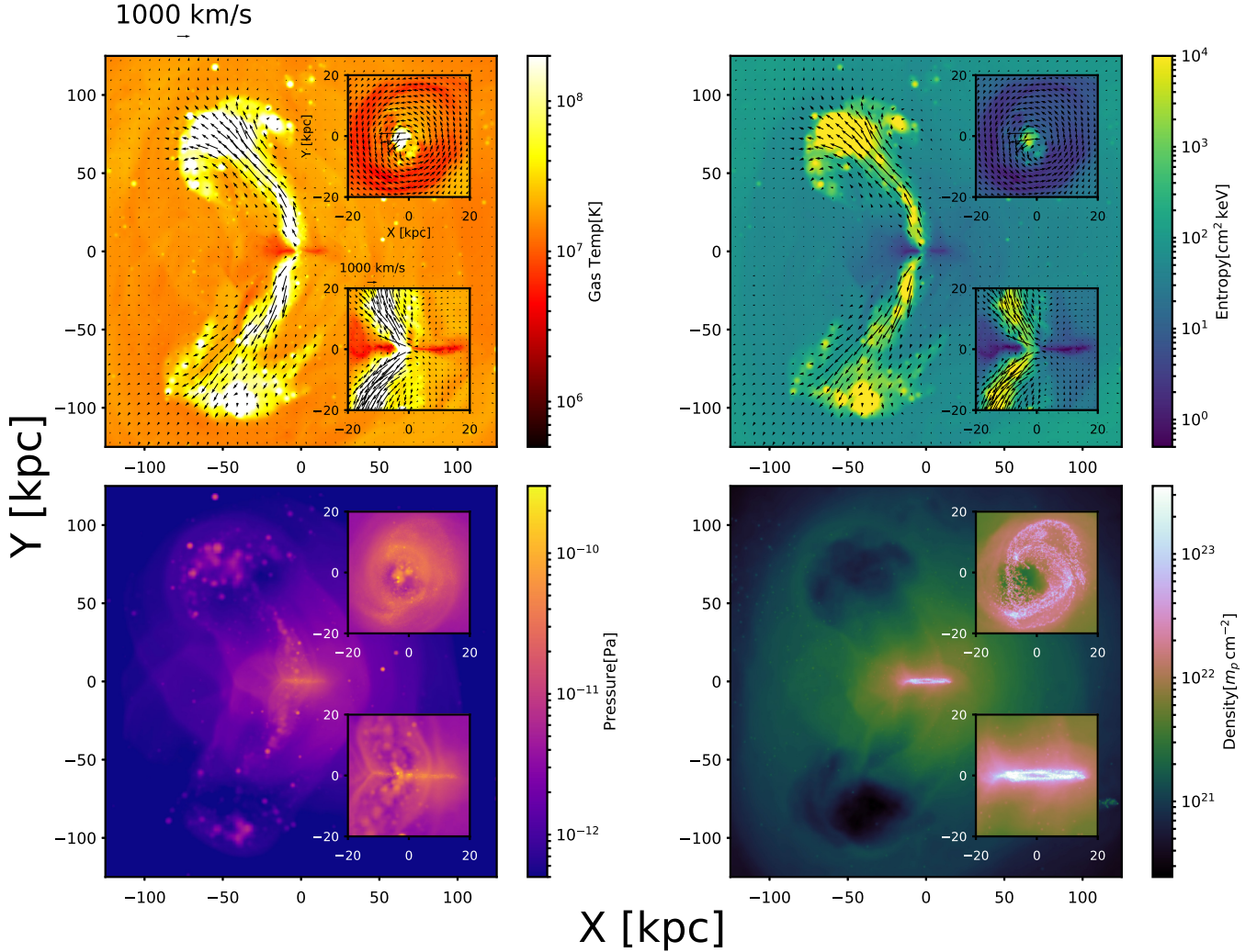
Figure 10. Outflows in action. Images of temperature (top left), entropy (top right), pressure (bottom left), and column density (bottom right) of cluster gas at z = 0.53 ( t = 8.41 ). Each large panel is a mass-weighted slice along a 30 kpc slice through the centre of the cluster. The inset panels are 5 kpc slices zooming into the central regions. The exception to this is the density plot, which is a 100 kpc slice for all panels in order to better show the structure of the gas. A large-scale outflow is clearly seen in the temperature and entropy plots, which also overlay the velocity field. The gas in the outflow is moving at 1000 \text{ km s}^{-1} . The structure of the outflow is less clear in the pressure plot; the outflow has a similar pressure as the ambient gas, which is how it is able to maintain its collimation. The tips of the outflow show a high-pressure, low-density region, which can be seen to create bubbles in the gas, similar to what is observed in X-ray cavities. Although the outflow is powerful, it coexists with low entropy, 10^6 \text{ K} , rotationally supported core. Shocks can be seen propagating through the inner regions in the pressure plot, helping to balance the cooling as seen in, e.g. Li et al. (2015).
