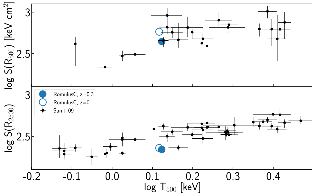
Figure 5. The entropy of the ICM. The observed relationship between entropy and overall cluster temperature. The blue points represent results from ROMULUSC at z = 0 (open) and z = 0.3 (solid). The entropy is measured within 1 kpc thick annuli at R_{2500} (bottom) and R_{500} (top). Like in Fig. 4, we take the average between mass- and emission-weighted values for temperature to calculate entropy. Again, only diffuse, hot gas is included in the analysis.
