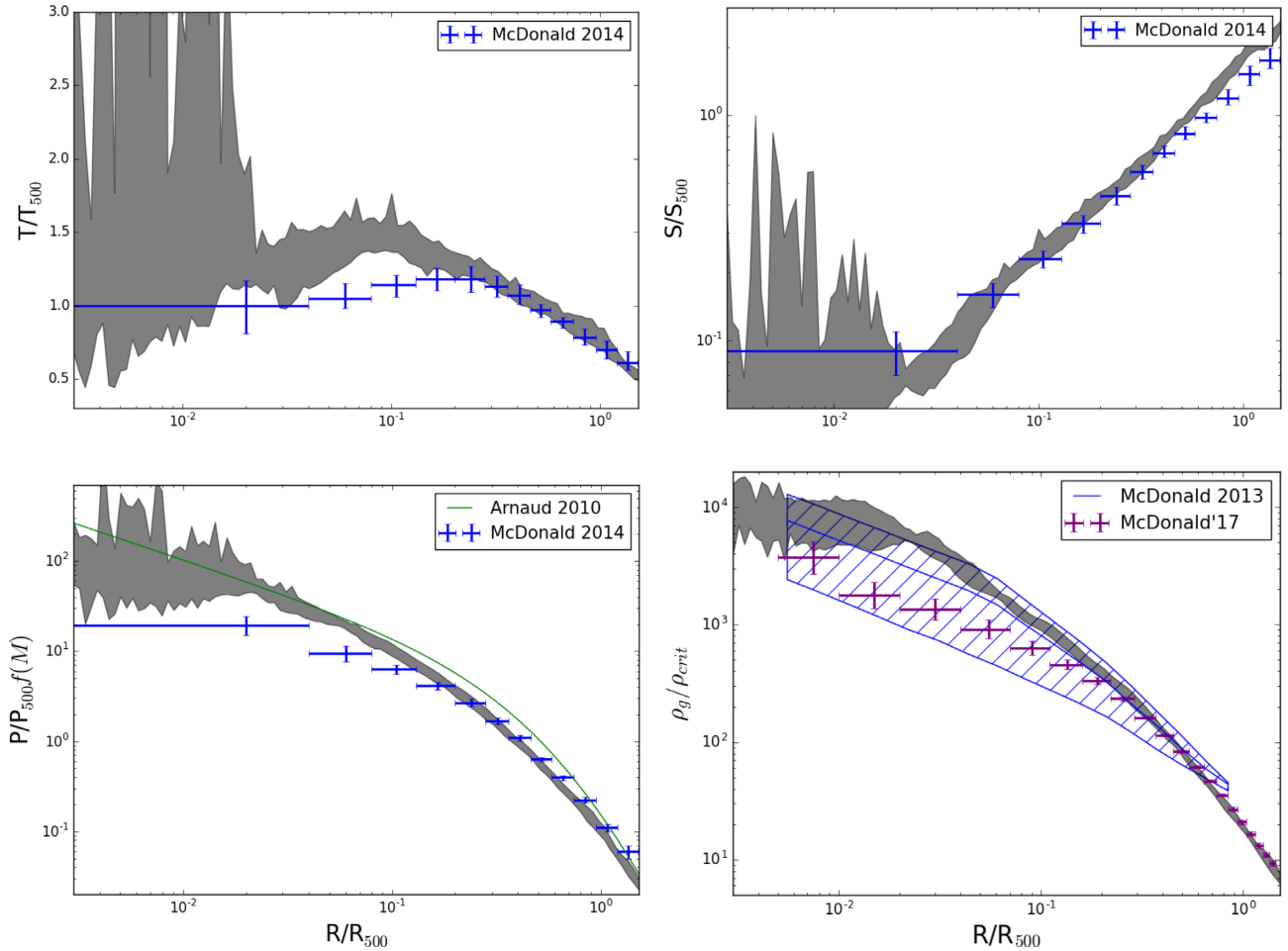
Figure 6. The structure of the ICM. Radial profiles of the temperature, entropy, pressure, and density of the ICM gas in ROMULUSC (grey bands). The grey bands correspond to the range of profiles from z = 0.3 – 0.5 . This redshift range was chosen because it corresponds to a period in the simulation prior to the late-time major merger where the cluster still has a cool core. It is also a similar redshift range as the clusters examined in McDonald et al. (2014). At z < 0.3 the in-falling group causes increasing disturbance away from equilibrium. As stated in the text, we will examine the effect of this merger on the ICM properties in future work. Overplotted are the results from McDonald et al. (2013, 2014, 2017). For pressure we also compare with results from Arnaud et al. (2010) which are at lower redshifts, but include more similar mass clusters to ROMULUSC. All observed data sets are selected to be cool-core clusters, except for the mean density profile from McDonald et al. (2017). Overall, ROMULUSC fits well with average profiles of cool-core clusters. Compared to McDonald et al. (2014) ROMULUSC has slightly high temperature and pressure within the inner 0.2R_{500} , but matches well with the Arnaud et al. (2010) results for pressure within 0.2R_{500} . The density profile matches well with the average profile for all clusters from McDonald et al. (2017), but deviates from self-similarity on small scales where it matches much better median density profile for clusters selected to have low-entropy cores (McDonald et al. 2013).
