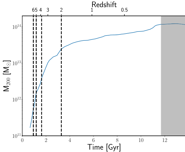
Figure 2. Growth of the ROMULUS cluster. The growth in halo mass of ROMULUS’s main progenitor over cosmic time. By z \sim 2 the main progenitor to ROMULUS is as massive as the most massive halo at z = 0 in our uniform volume simulation, ROMULUS25. Thus, ROMULUS represents a unique environment in which to examine galaxy evolution and an important addition to our simulation suite. Mergers of total mass ratio 1:10 or higher are shown as vertical dashed lines. The grey band represents the ongoing merger starting around z = 0.17 , which has a 1:8 total mass ratio and a 1:2 stellar mass ratio. In some of our analysis we will ignore the time period associated with this merger.
