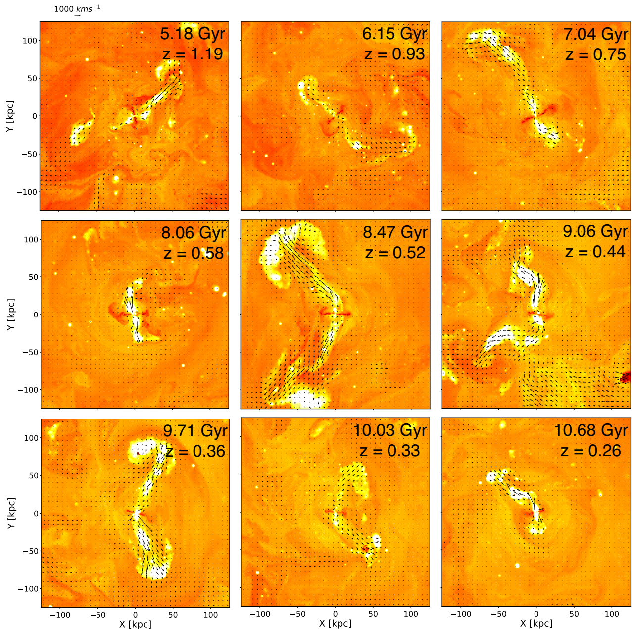
Figure 11. AGN-driven outflows over time. Snapshots of the gas temperature and velocity field in the inner regions of ROMULUSC over cosmic time. Each image shows the same projection, modulo rotations about the y-axis in order to best image capture any outflow structures present. The colours are the same as Fig. 10. The temperatures are mass-weighted averages along a 2 kpc slice centred at halo centre. It is clear that the winds evolve in direction, shape, and magnitude. The direction is dictated by the rotation of gas in the inner 10–20 kpc of the halo as well as the larger scale motions of the ICM. Between 8 and 10 Gyr, the outflows are particularly strong, corresponding to a period of both high SMBH activity and declining star formation in the BCG (see Fig. 9).
