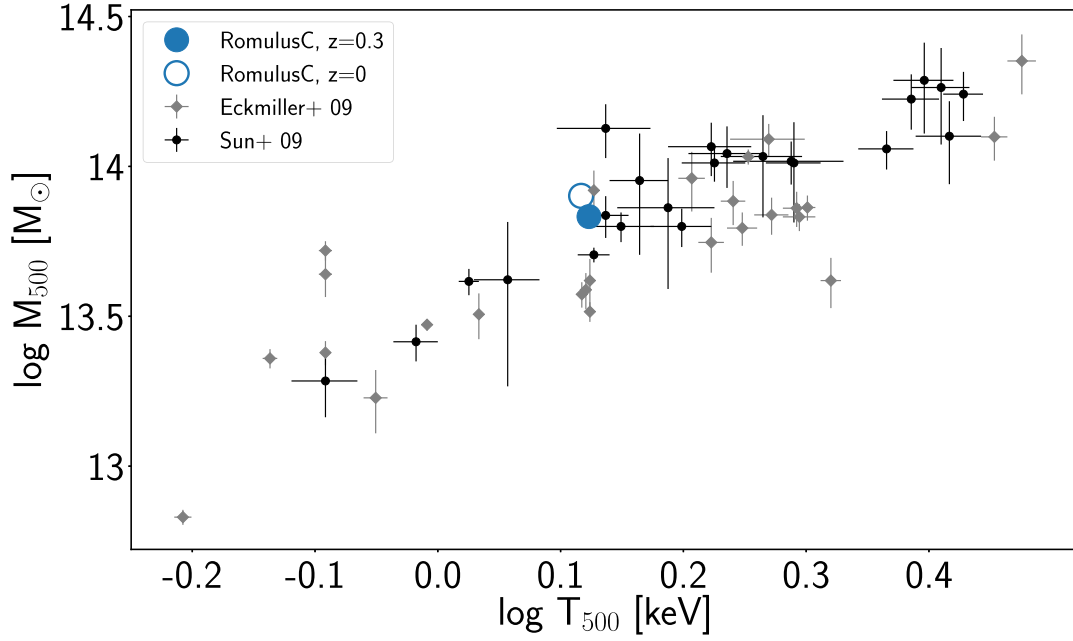
Figure 4. The temperature of the ICM. The observed relationship between group and cluster masses ( M_{500} ) and the core-excised temperature, T_{500} . The open blue circle represents ROMULUSC at z = 0 and the solid circle at z = 0.3 , when the cluster is still in equilibrium prior to the in-fall of a galaxy group and what will be an on-going merger at z = 0 . To calculate the temperature we use an average between the emission-weighted and mass-weighted results for diffuse ( \rho < 500\rho_{\text{crit}} ), hot gas detectable by X-ray observatories ( T > 0.1 keV). This decision is based on results from Liang et al. (2016) showing that this average better approximates results from more detailed spectroscopic models at this mass scale and are therefore closer to what an observer would see. Our results are insensitive to this choice.
