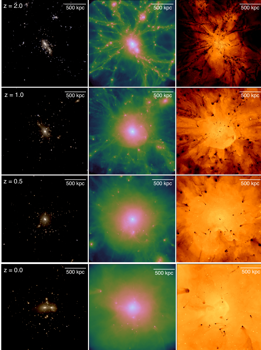
Figure 1. Evolution of gas and stars in ROMULUSC. Four snapshots of ROMULUSC taken (from the top) at z = 2, 1, 0.5 , and 0 showing stars (left-hand side), gas column density (middle), and gas temperature (right-hand side). The temperature is averaged along the line of sight and weighted by \rho^2 . All of the plots show the same physical region encompassing what will be R_{200} at z = 0 (the scales are also in physical units). The stars are shown in UVJ colours assuming a Kroupa IMF. The density ranges from 1 \times 10^{-5} \text{ g cm}^{-2} (blue/black) to 0.1 \text{ g cm}^{-2} (pink/white). The temperature ranges from 5 \times 10^4 \text{ K} (black) to 5 \times 10^8 \text{ K} (yellow). At early times there are a lot of cold gas filaments penetrating the halo, which triggers more star formation in cluster galaxies. At later times, the halo is massive enough to prevent such filaments from penetrating far into the halo. Ram pressure stripping is evident in the extended tails of cold gas in the cluster galaxies. At z = 0 there are two galaxies interacting near the centre. The less massive of the two, which makes its first pericentre passage into the centre of the cluster around z = 0.17 , is half the stellar mass of the BCG and comes from a halo one eighth the mass of the main halo.
