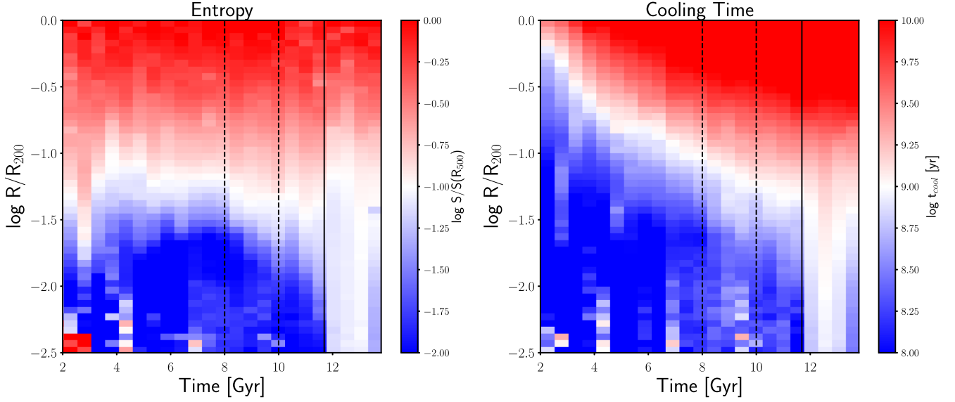
Figure 13. Survival of the cool core. Entropy and cooling time profiles as a function of time for ROMULUSC. Up until the onset of a major merger, marked by the vertical black line, the entropy profile remains steeply declining towards the centre of the halo and the cooling times remain below 1 Gyr, both important characteristics of a cool-core cluster. Between 8 and 10 Gyr, the star formation and amount of cold gas in the central regions declines due to the large-scale AGN feedback, but the cluster maintains a low-entropy core with sub-Gyr cooling times. Following the major merger, the entropy profile flattens out and the cooling times become several Gyr, consistent with non-cool-core systems.
