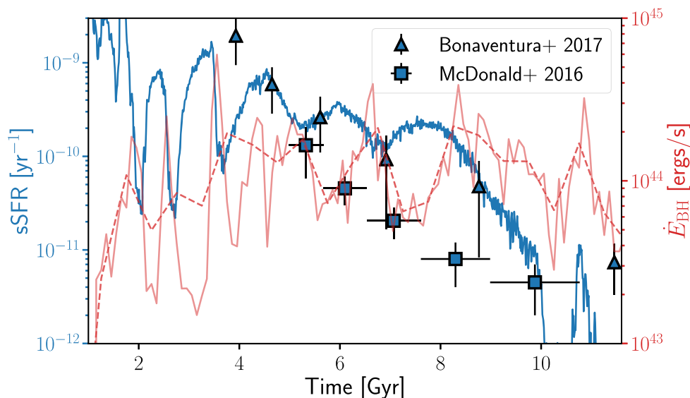
Figure 9. Star formation and SMBH feedback history. The specific star formation rate (blue, averaged over 10 Myr bins) and feedback rate of the central SMBH (red, averaged over 100 and 500 Myr bins for solid and dashed lines, respectively) for the BCG in ROMULUSC. The SMBH feedback traces both accretion and feedback energy imparted by the SMBH on to nearby gas. Dips in the sSFR are often associated with peaks of SMBH activity. The peak of activity beginning around 8 Gyr and persisting through 10 Gyr is associated with the final quenching of the BCG. The sSFR history of the ROMULUSC BCG is remarkably close to the average evolution observed in clusters from Bonaventura et al. (2017), but slightly high compared to results from McDonald et al. (2016). The range in time shown is cut off just prior to the infall of the group seen in Fig. 7. The merger destroys the cool core, a topic to be explored in future work.
