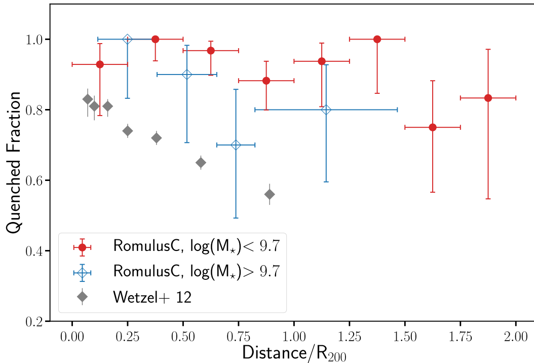
Figure 15. Quenching as a function of position in a cluster. The quenched fraction as a function of distance from halo centre for two mass bins. At high mass (blue, open points; chosen to match the masses of observed cluster galaxies from Wetzel et al. 2012) our values are high compared with observations, but as explained in the text this is due to the lowest mass galaxies in this bin. At low masses we predict that no trend exists. At all radial distances low-mass galaxies have a quenched fraction of 80–90 per cent. Error bars represent the 68 per cent binomial confidence interval (Cameron 2011).
