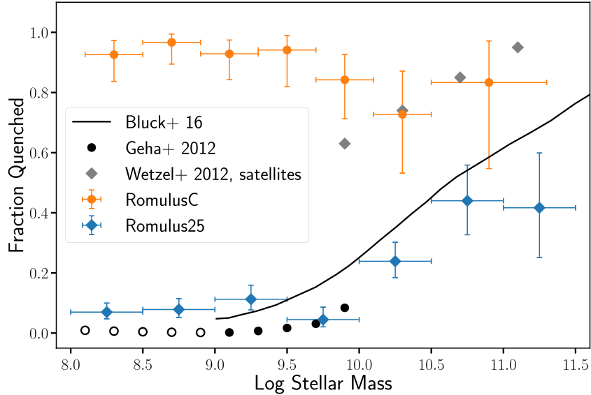
Figure 14. Quenching as a function of stellar mass. The fraction of quenched galaxies as a function of stellar mass for both ROMULUSC (orange points) and ROMULUS25 (blue diamonds). At all but the highest masses we find that satellite galaxies in ROMULUSC have a much higher quenched fraction than isolated galaxies. Our results are consistent with the quenched fraction found by Wetzel et al. (2012), but due to small number statistics we cannot confirm that we also see a trend at high mass. At low masses we find the quenched fraction remains nearly constant at 80–90 per cent. Error bars represent the 68 per cent binomial confidence interval (Cameron 2011). The open points are also from Geha et al. (2012) and represent upper limits.
