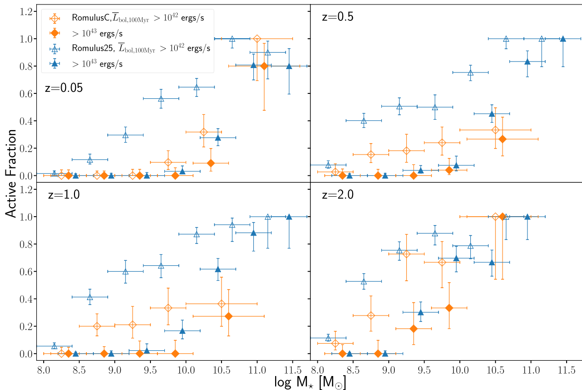
Figure 19. The population of luminous AGN. The fraction of galaxies hosting SMBHs that have a luminosity above a threshold of 10^{42} (open points) and 10^{43} (closed points) \text{erg s}^{-1} as a function of stellar mass at four different redshifts. Luminosities are averaged over the previous 100 Myr. Note that we do not include z = 0 because the black hole properties are only followed to z = 0.05 in ROMULUS25. Low-luminosity AGN are much more affected by their environment while high-luminosity AGN, which occur only in more massive galaxies, seem relatively insensitive to being in a cluster versus relatively isolated galaxy. Both AGN fractions evolve significantly with redshift such that, by z = 2 , both are very similar to the field. This is in contrast with Fig. 18, which shows a substantial population of very low Eddington ratio SMBHs. When only focusing on high luminosity (which means high accretion rate) much of the difference in environment seen in the Eddington ratio vanishes, leading to claims that observed high-redshift AGN population in clusters are similar to or even enhanced compared with the field. Error bars represent the 68 per cent binomial confidence interval (Cameron 2011).
