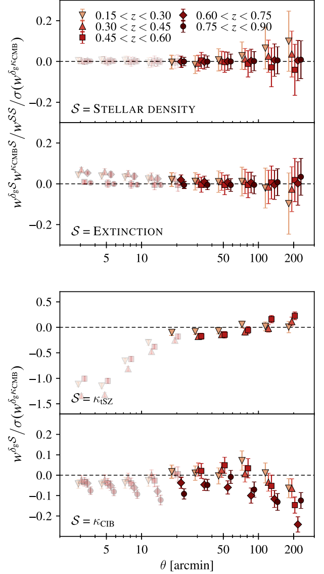
FIG. 2. Top two panels: Contributions due to uncorrelated systematics to the galaxy-CMB lensing cross-correlations, as described by Eq. (23), in units of the statistical errors on the observed cross-correlation. Lower two panels: Contributions due to correlated systematics, given by the cross-correlations between the \kappa_{\text{CMB}} systematics ( \kappa_{\text{tSZ}} and \kappa_{\text{CIB}} ) and \delta_g , also in units of the statistical error. We observe that within the angular scales we consider the ratios are < 1 for all redshift bins for all systematic maps (the faded points are removed from the analysis due to the imposed scale cuts). Since the tSZ template is generated only using REDMAPPER clusters up to z = 0.6 , the correlations for the higher two redshift bins have been ignored (see [44]). Note the different scales used for \kappa_{\text{tSZ}} and \kappa_{\text{CIB}} .
