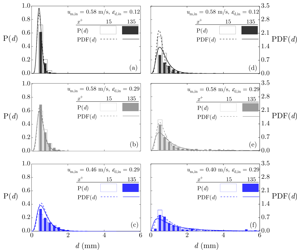
FIG. 6. Probability histograms and the log-normal probability density functions for the flow conditions of Fig. 2 for both o/w (a)–(c) and w/o (d)–(f) dispersions.
