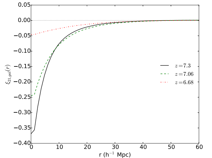
Figure 7. Theoretical 3D 21 cm-galaxy cross-correlation function at z = 6.68 (red dash-dotted line), 7.06 (green dashed) and 7.3 (black). The black dotted line indicates zero correlation.
