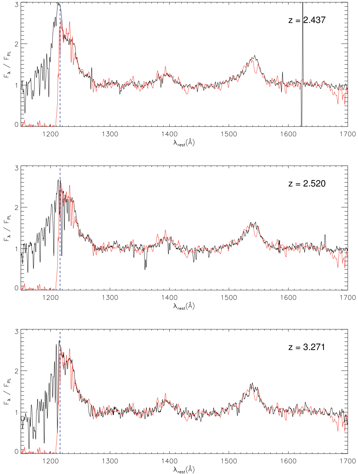
Figure 6. SDSS spectra of objects at lower redshifts which match J1120+0641’s spectrum in C iv as well all the way to the onset of the Lyman \alpha forest at 1216 Å, indicated by the blue dashed line. The GNIRS spectrum of ULAS J1120+0641, binned in bins of three, is overlaid in red. All spectra are normalized by a fitted power law. SDSS spectra are binned in bins of five. The C iv parameters of these objects are shown as green dots on Fig. 4.
