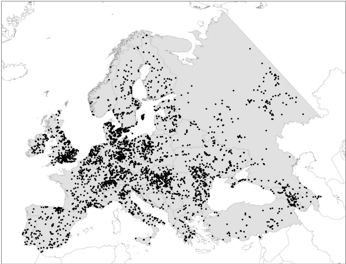
Figure S1. Map of Europe showing the spatial distribution of zooarchaeological large mammal records from the Holocene.
