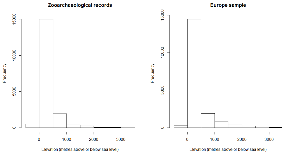
Figure S2. Elevation profiles for c. 18,500 Holocene zooarchaeological records in Europe (left) and randomly sampled from an ArcMap layer of European elevation (right).
