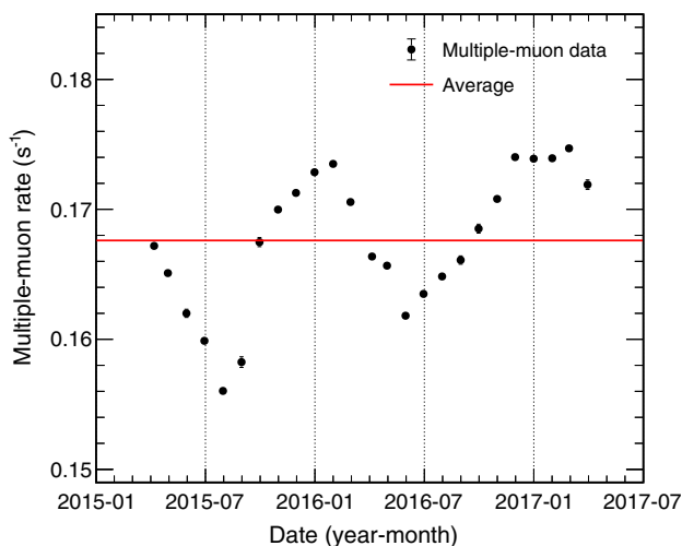
FIG. 3. Rate of multiple muons in the NOvA ND as a function of month and year.
