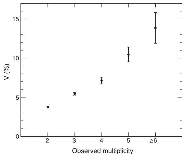
FIG. 10. Fitted amplitudes (%) to a cosine fit of the seasonal variation for each observed multiplicity in the NOvA ND.
