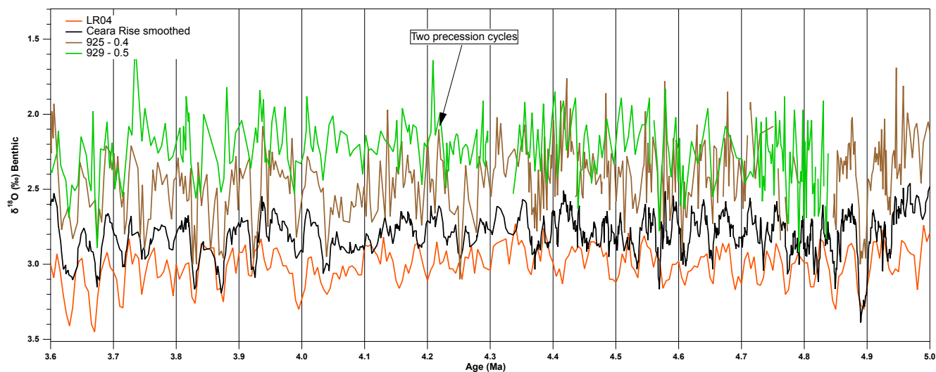
Figure 12. A comparison of LR04 and Ceara Rise (smooth) to Site 925 and Site 929 benthic isotope data. LR04 assignment of variability in the interval from 4.0 to 4.5 Ma to precession peaks may have resulted in the mismatch with the Ceara Rise stack.
