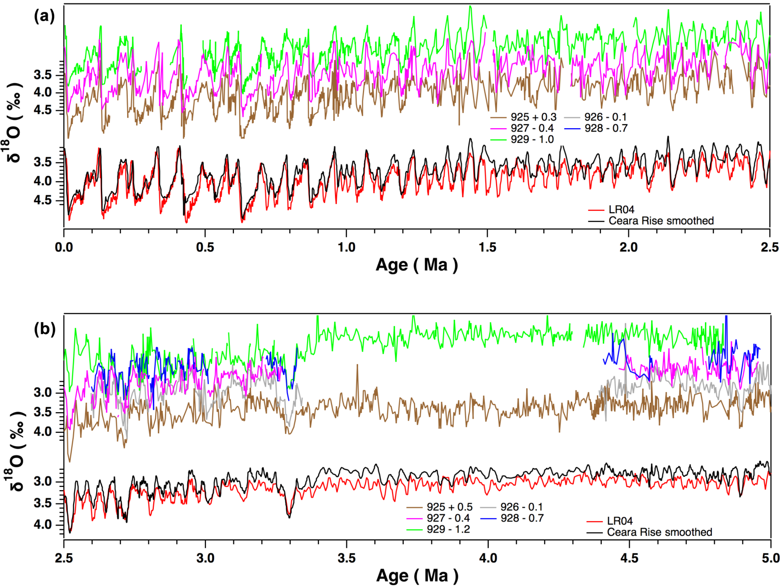
Figure 8. Benthic oxygen isotope data from all Ceara Rise sites compared with one another and a smoothed composite of all data compared to LR04. (a) 0 to 2.5 Ma; (b) 2.5 to 5 Ma. Note the \delta^{18}\text{O} scale change between (a) and (b). Individual site traces have been offset as indicated in the legend.
