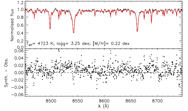
Figure 3. Top: observed (in black) and synthetic (in red) spectra of a RAVE super metal-rich star. Bottom: residuals between the observations and the synthetic spectrum. [A colour version of this figure is available in the online version.]
