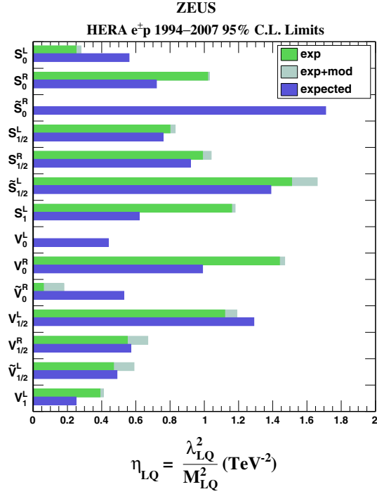
FIG. 5. Upper 95% C.L. limits on the LQ coupling strength, \eta_{LQ} = \lambda_{LQ}^2/M_{LQ}^2 . Compared are the limits calculated without (dark upper bars) and with (light upper bars) modeling uncertainties, and the expected limits (lower bars).
