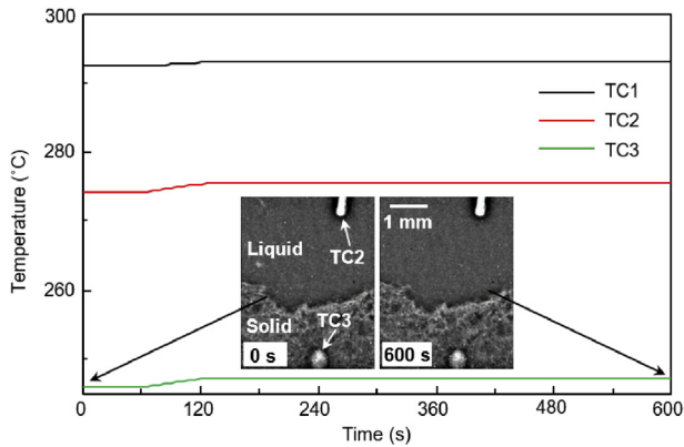
Fig. 3. The temperature profiles recorded during the cooling processes of the Bi-8% Zn alloy. The insets show the X-ray images of the L-S interface before and after continuously exposed to the X-ray beam for 600 s at Beamline I12. The white solid particles are the primary Zn phases.
