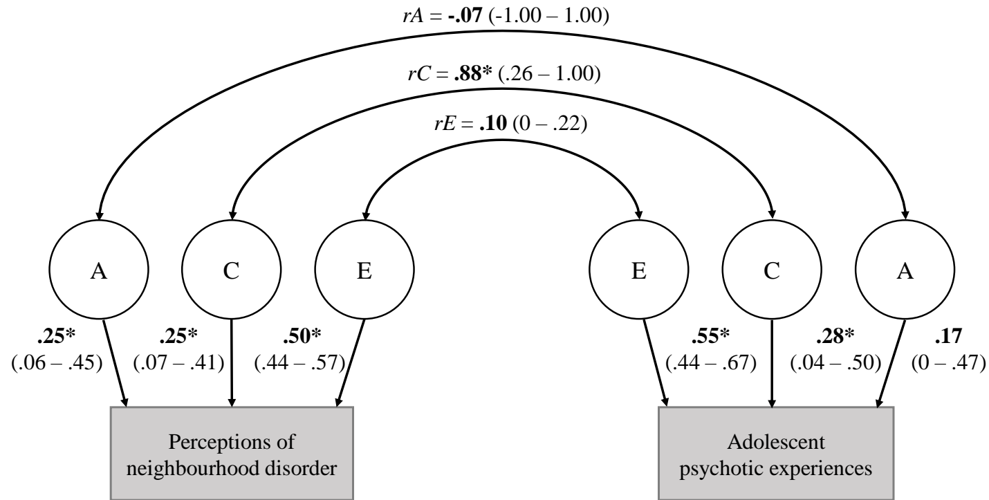
Figure 1 ACE estimates and ACE correlations from cross-twin cross-trait (bivariate) model
