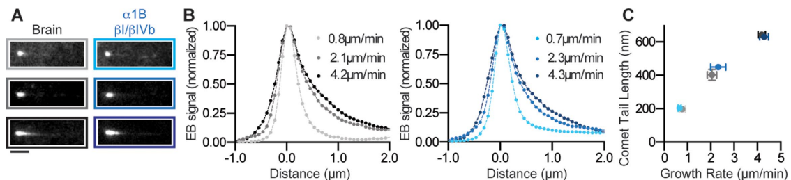
FIGURE 4: EB1-GFP comet analysis on brain and \alpha 1B/ \beta 1+ \beta IVb microtubules. (A) TIRF microscopy images of EB1-GFP comets at the ends of growing brain microtubules (left) and \alpha 1B/ \beta 1+ \beta IVb (right) microtubules at different growth speeds. From top to bottom: brain microtubule growth speeds are 0.8, 2.1, and 4.2 \mu m/min ( n = 26, 13, and 15 microtubules, respectively). From top to bottom: \alpha 1B/ \beta 1+ \beta IVb microtubule growth speeds are 0.7, 2.3, and 4.3 \mu m/min ( n = 24, 12, and 10 microtubules, respectively). Scale bar: 2 \mu m. (B) Averaged fluorescence intensity profiles of EB1-GFP comets at different growth speeds of brain (left) and \alpha 1B/ \beta 1+ \beta IVb (right) microtubules. n = 420, 333, and 421 comet profiles from 12, 13, and 15 brain microtubules at growth speeds of 0.8, 2.1, and 4.2 \mu m/min, respectively and n = 364, 351, and 234 comet profiles for 15, 12, and 10 \alpha 1B/ \beta 1+ \beta IVb microtubules at growth speeds of 0.7, 2.3, and 4.3 \mu m/min, respectively. (C) EB1-GFP comet tail lengths as a function of microtubule growth speeds for brain (gray) and \alpha 1B/ \beta 1+ \beta IVb (blue) microtubules. Comet tail lengths were obtained by single exponential fits to the averaged intensity profiles (see Materials and Methods ).
