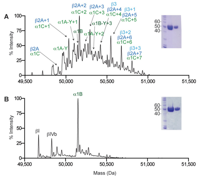
FIGURE 1: Isoform composition and purity of tubulin isolated from brain tissue and tsA201 cells using the TOG affinity method. (A) Mass spectra and SDS–polyacrylamide gel (inset) of tubulin isolated from mouse brain. Number of posttranslationally added glutamates is indicated for the glutamylated species. (B) Mass spectra and SDS–polyacrylamide gel (inset) tubulin isolated from tsA201 cells (see Materials and Methods ).
