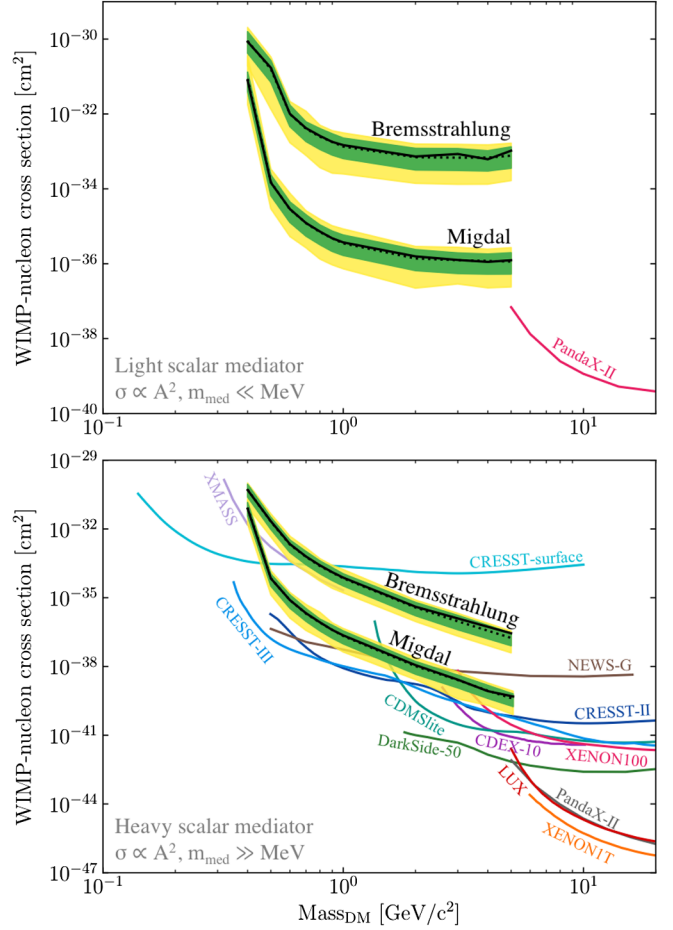
FIG. 6. Upper limits on the SI DM-nucleon cross section at 90% C.L. as calculated using the bremsstrahlung and Migdal effect signal models assuming a scalar mediator (coupling proportional to A^2 ). The 1- and 2- \sigma ranges of background-only trials for this result are presented as green and yellow bands, respectively, with the median limit shown as a black dashed line. The top figure presents the limit for a light mediator with q_{\text{ref}} = 1 \text{ MeV} . Also shown is a limit from PandaX-II [10] (pink), but note that Ref. [10] uses a slightly different definition of F_{\text{med}} in their signal model. The bottom figure shows limits for a heavy mediator along with limits from the SI analyses of LUX [1] (red), PandaX-II [2] (gray), XENONIT [28] (orange), XENON100 S2 -only [29] (pink), CDEX-10 [30] (purple), CDMSlite [31] (teal), CRESST-II [32] (dark blue), CRESST-III [33] (light blue), CRESST-surface [34] (cyan), DarkSide-50 [35] (green), NEWS-G [36] (brown), and XMASS [37] (lavender).
