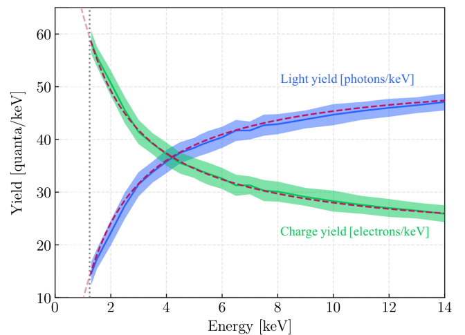
FIG. 1. The light (blue) and charge (green) yields of tritium ER events as a function of recoil energy as measured in situ by the LUX detector at 180 V/cm (solid lines) compared to NEST v2.0 simulations (dashed pink line). The bands indicate the 1\text{-}\sigma systematic uncertainties of the measurement. The dotted gray line shows the 1.24 keV energy threshold implemented in the analysis.
