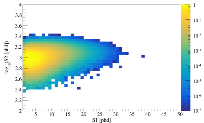
FIG. 4. The expected signal from DM-nucleus interactions through the Migdal effect with a cross section per nucleus of 1 \times 10^{-35} \text{ cm}^2 projected onto a two-dimensional space of \log_{10}S2 vs S1 . Assumptions are the same as in Fig. 3 with additional data quality cuts applied.
