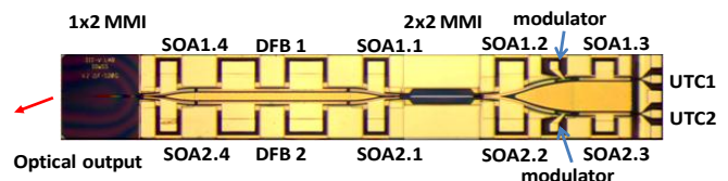
Fig. 1: Microscope view of the dual DFB dual wavelength source
