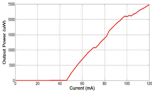
Fig. 8: L-I characteristic curve at the the channel output on a Type B channel. As the channel SOA is biased, the phase shifter remains in open circuit.
