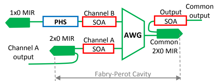
Fig. 2. Schematic of the AWG laser dual wavelength source showing the two types of channels: Type A, with SOA and Type B with SOA and PHS.
