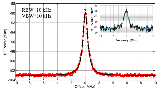
Fig. 11: Optical linewidth with channel SOA current at 50 mA and Boost SOA at 60 mA. The inset shows the beat note with adjacent channel at 80 mA.
