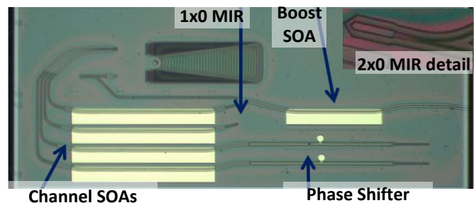
Fig. 3. Microscope view of the fabricated AWG laser dual wavelength source
