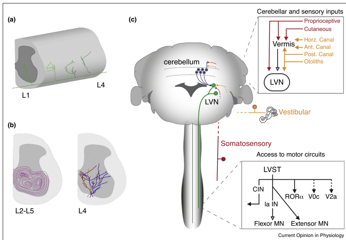
Branching pattern of individual LVST-neurons and integration within the locomotor system. (a) Branching pattern of a single LVST-axon at multiple segmental levels of the lumbar spinal cord. (b) Left—density plot showing position of synaptic puncta from LVST-neurons in the lumbar spinal cord. Right—overlay of four separate LVST-axons at lumbar level four. (c) Summary of LVST-neurons in the locomotor control system, showing sensory and cerebellar input and output to defined classes of spinal interneuron. Upper inset shows cerebellar and vestibular input to the LVN. Lower inset shows known connections between LVST-neurons and spinal interneurons. Panels A and B (right) adapted from Figure 8 in Kuze et al. [68]; Panel B (left) adapted from supplementary Figure 8 in Murray et al. [9]. Abbreviations: Ant. – Anterior; CIN – Commissural interneuron; Horz. – Horizontal; IN – Interneuron; L – Lumbar level; LVST – Lateral vestibulospinal tract; Post. – Posterior.
