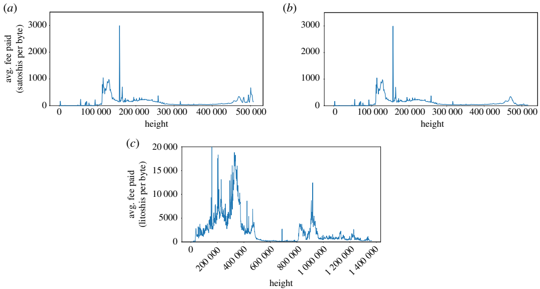
Figure 8. Average fee rate (in satoshis/litoshis per byte) paid by transactions at a given block height. The plot is showing 1000 block averages. (a) Bitcoin, (b) Bitcoin Cash and (c) Litecoin.
