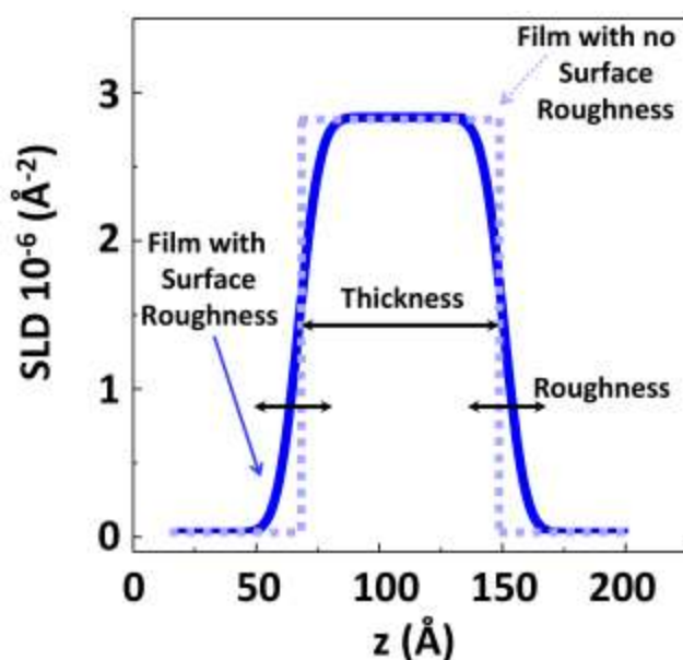
Figure S2. Schematic of a SLD profile in which are highlighted thickness and surface roughness. In the plot are compared SLD profiles for an ideal and a real sample having the same layer thickness. The ideal profile corresponds to a roughness-free sample (dashed line); the real sample is the one with a non-zero surface roughness (solid line).
