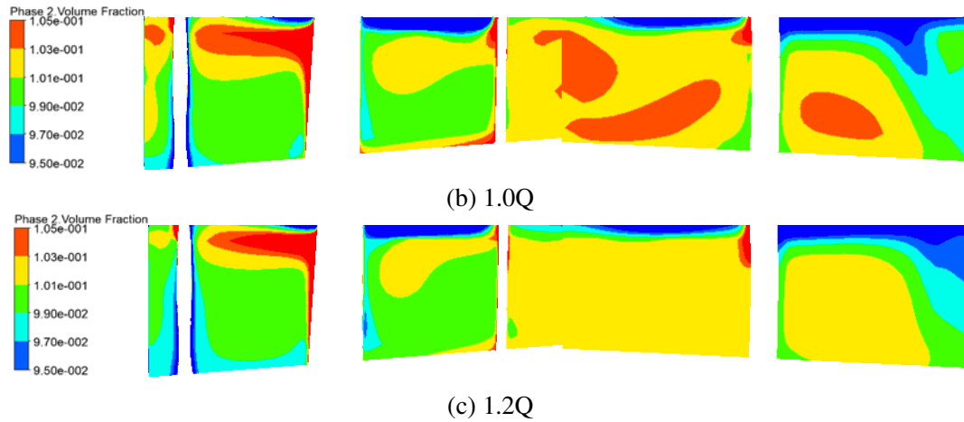
Figure 2. IGVF=0.1 the axial of the gas volume distribution within the multiphase pump first compression unit under the different flows
