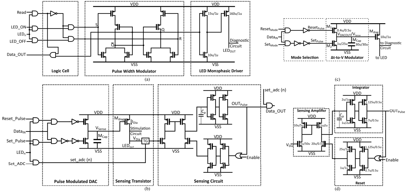
Fig. 6. (a) Circuit schematic of stimulation control block. LED ON /LED OFF signals determine the operation status of emitters. Read signal monitors the real-time working state saved by PWM unit. (b) A circuit schematic of diagnostic sensing block. Set_Pulse and Reset_Pulse generate pulse signals to achieve voltage scanning. Set_ADC determines the timing control of the \Sigma\Delta ADC to fetch the V Di a . (TG is short for transmission gate). (c) Circuit schematic of the pulse width modulated DAC. This DAC performs two operations: mode selection and time-to-voltage conversion. (d) The diagnostic sensing element. Left is a (non-OTA) transconductance amplifier which feeds current into a simple \Sigma\Delta ADC (right). This consists of three stages: current buffering, integration, and reset/pulse control.
