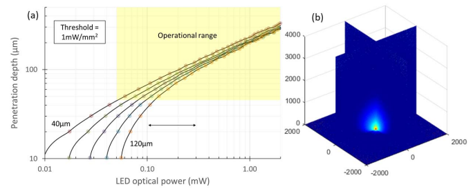
Fig. 3. Light transmission in tissue (a) the optical power required for a Lambertian emitting LED to reach a certain penetration depth for a 1 mW/mm 2 threshold. This is given for different emission region diameters from 40 \mu\text{m} to 120 \mu\text{m} . (b) the 3D profile of light penetration through tissue.
