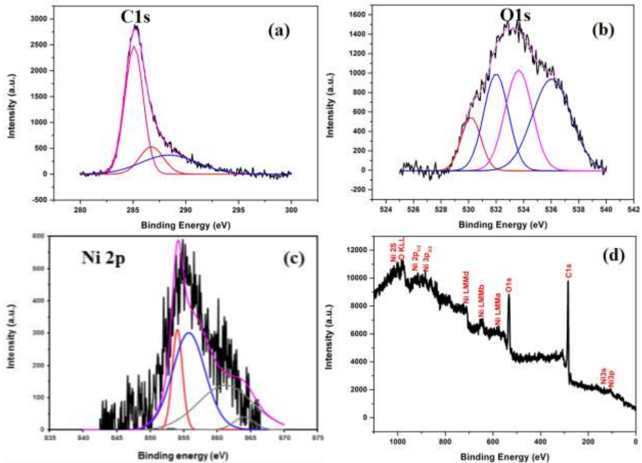
Fig. 2 XPS spectra of NiO/NPC a) C1s, b) O1s, c) Ni 2p, and d) survey scan spectrum of NiO/NPC
