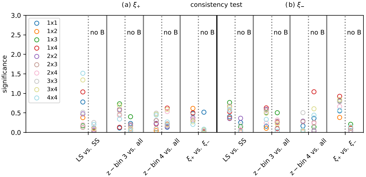
Figure D3. Significances for tension estimated by comparing the differences of the joint and split TPDs to zero for the following splits of the fiducial KiDS-450 data vector (from left to right): large versus small scales ('LS versus SS'), z-bin 3 and all its CCs versus all other z-bin combinations ('z-bin 3 versus all'), z-bin 4 and all its CCs versus all other z-bin combinations ('z-bin 4 versus all'), ' \xi_+ versus \xi_- '. (a) Using the \xi_+ estimator only and per tomographic bin combination i \times j . (b) Using the \xi_- estimator only and per tomographic bin combination i \times j . The columns marked with 'no B' use the KiDS-450 data vector from which the measured small-scale B modes were removed.
