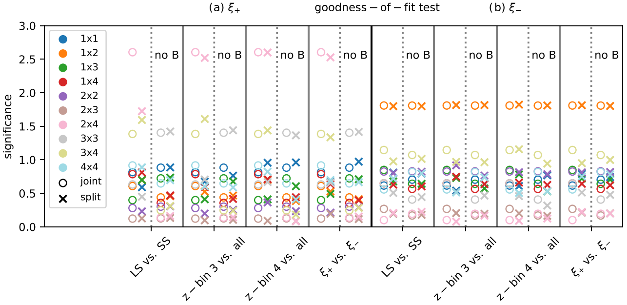
Figure D2. Significances for the goodness of fit estimated by comparing the joint (open circles) and split TPDs (crosses) to the data distribution for the following splits of the fiducial KiDS-450 data vector (from left to right): large versus small scales ('LS versus SS'), z-bin 3 and all its CCs versus all other z-bin combinations ('z-bin 3 versus all'), z-bin 4 and all its CCs versus all other z-bin combinations ('z-bin 4 versus all'), ' \xi_+ versus \xi_- '. (a) Using the \xi_+ estimator only and per tomographic bin combination i \times j . (b) Using the \xi_- estimator only and per tomographic bin combination i \times j . The columns marked with 'no B' use the KiDS-450 data vector from which the measured small-scale B modes were removed.
