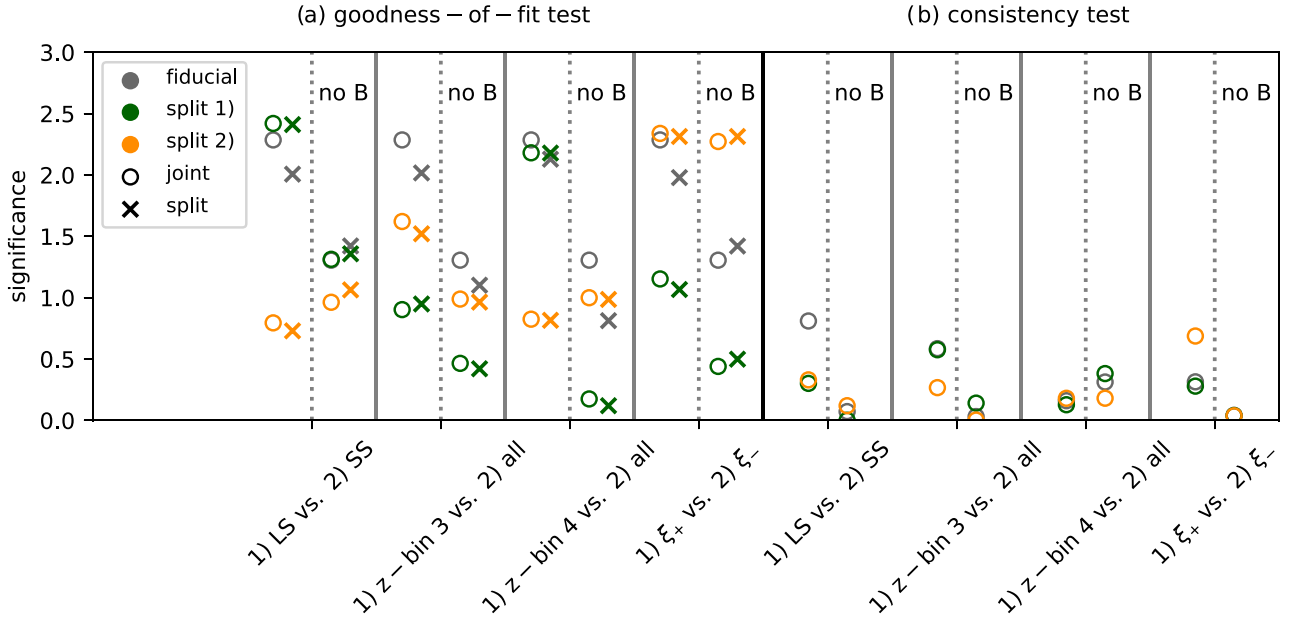
Figure 8. Significance as derived with the two TPD-based consistency estimators for different splits of the KiDS-450 data vector. (a) The significances for the goodness of fit are estimated by comparing the data distribution to the joint (circles) and split (crosses) TPDs. Grey symbols indicate that all fiducial angular scales (Table 1) are used in the significance estimation, whereas green and orange symbols correspond to one of the mutually exclusive subsets as indicated in the labels and along the x -axis. Shown are also the results when the measured B modes are subtracted from the data vector (‘no B’). (b) The significances for tension are estimated by comparing the differences between the joint and the split TPDs.
