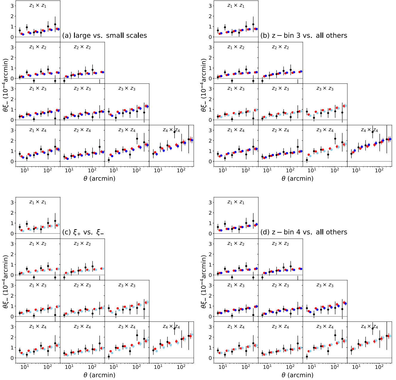
Figure D1. KiDS-450 data vector (black points) and TPD means (red and blue points) for the \xi_{-} estimator as a function of angular scale per redshift bin combination. The TPDs are based on the joint (red points; the same in all panels) and split (dark and light blue points) cosmological and nuisance parameters from MCMC runs fit to the data vector. The panels consider various mutually exclusive splits of the data vector (a) large versus small scales, (b) z-bin 3 (and all its CCs) versus all other redshift correlations, (c) \xi_{+} versus \xi_{-} , and (d) z-bin 4 (and all its CCs) versus all other redshift correlations. Error bars on the means are derived from the 68 per cent credibility interval around the mean. The error bars for the data are based on the diagonal of the covariance matrix.
