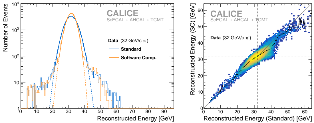
Figure 7. Reconstructed energy distributions from standard and software compensation reconstructions for the 32 \text{ GeV}/c \pi^- data. The black markers in the correlation plot show the profile of the mean software compensation reconstructed energy for bins of the standard reconstruction energy (right). The black dashed lines in the correlation plot indicate the beam energy of the sample.
